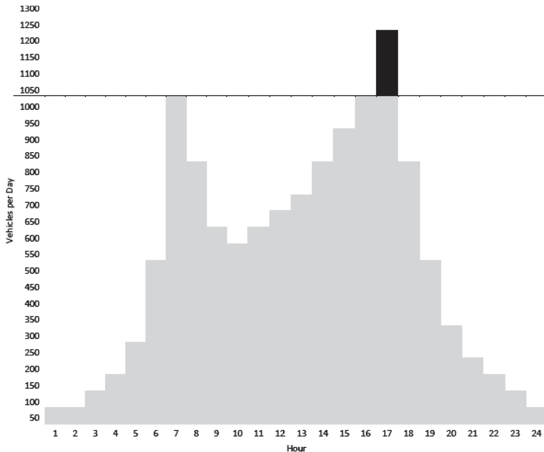
Figure 8-8. Peak-spreading example, first iteration over-capacity traffic.
