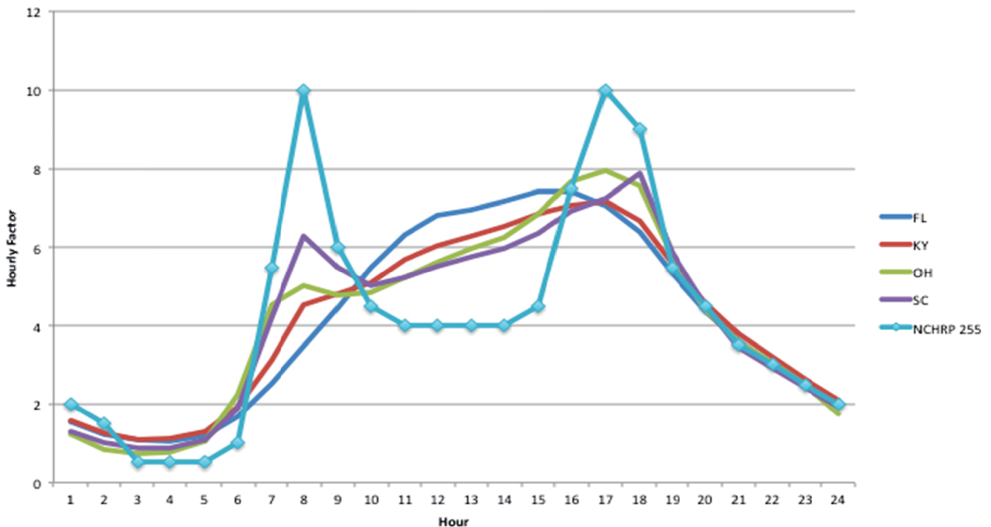
Figure 8-16. Hourly volume distribution for urban Interstates.
