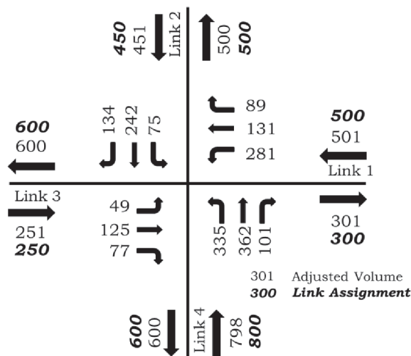
Figure 6-11. Turning movement forecasts.
