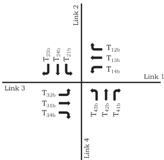
Figure 6-5. Iterative procedure—turning movements known.
