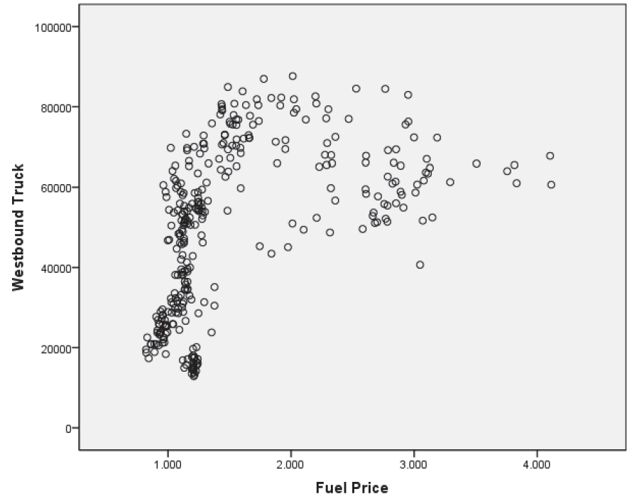
Figure 11-31. Scatterplot of westbound truck traffic and fuel price.
