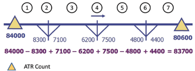
Figure 5-1. Example imbalance between upstream and downstream traffic counts with ramp entrance and exit volumes.
