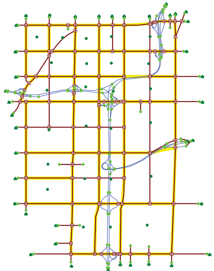
Figure 11-10. Milwaukee/Mitchell window network.
