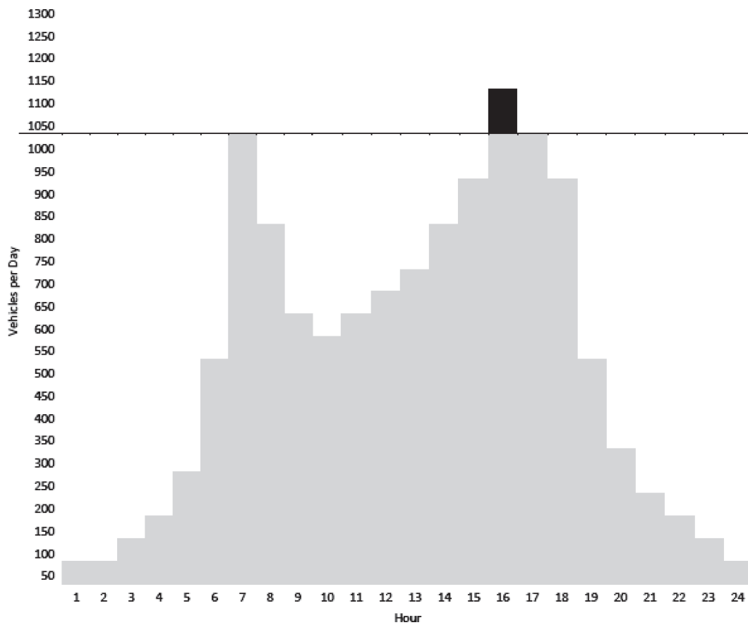
Figure 8-11. Peak-spreading example, second iteration over-capacity traffic.
