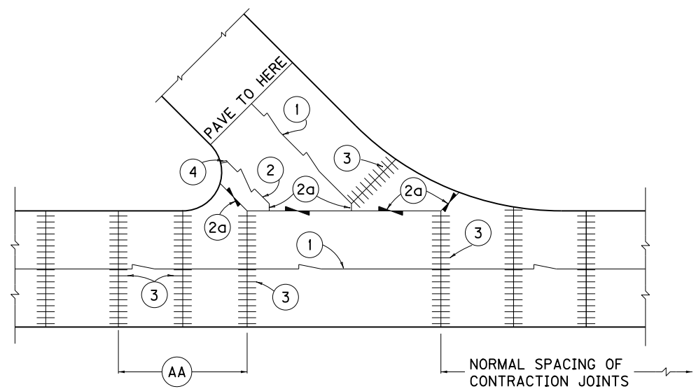
ANGLE INTERSECTION
