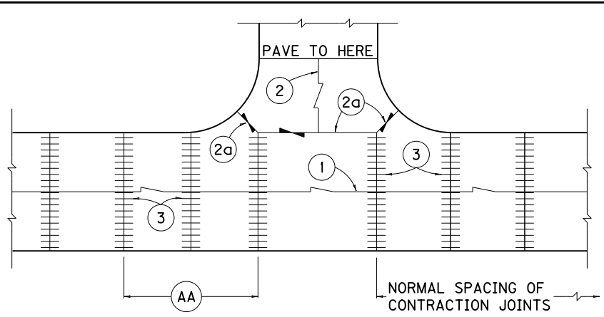
SINGLE INTERSECTIONS
