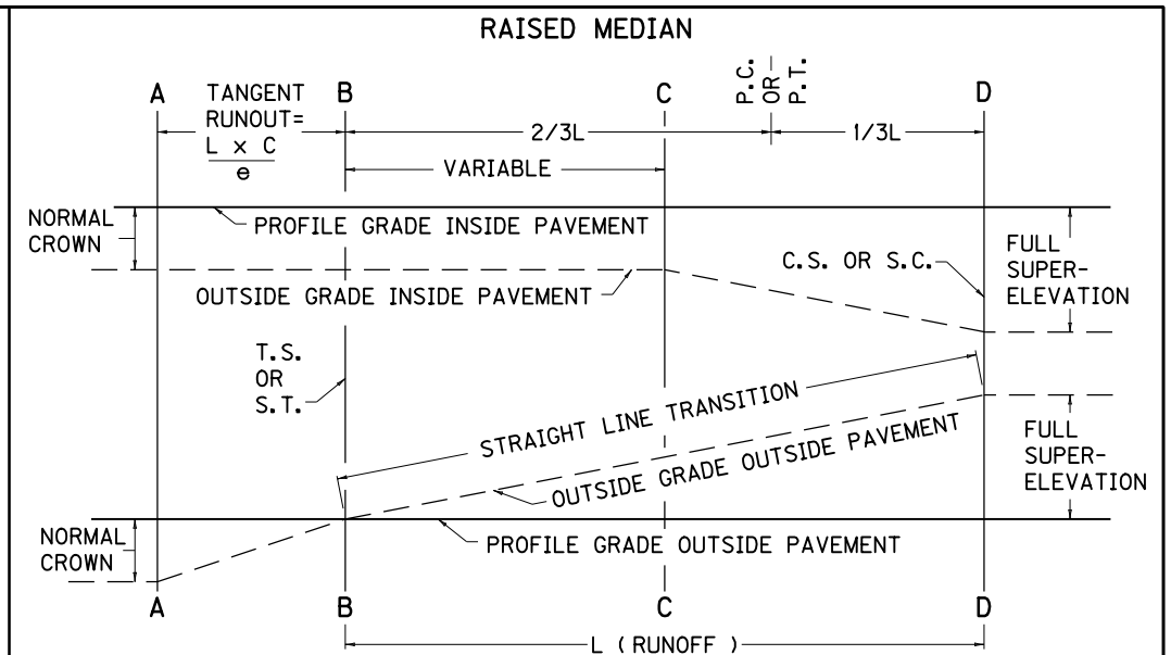
PROFILE OF PAVEMENT EDGES
