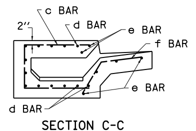
STANDARD CURB
