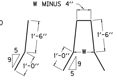
DETAIL OF "A" BAR DETAIL OF "B" BAR
