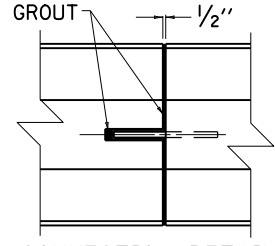
CONNECTION DETAIL
