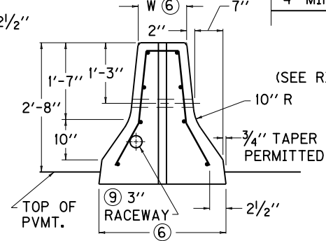
RIGHT ELEVATION VIEW
