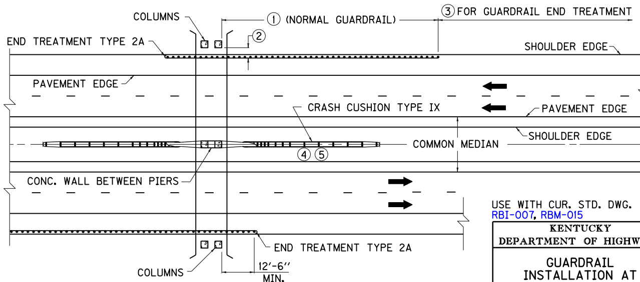
LOCATION OF GUARDRAIL WITH CONSTANT WIDTH MEDIAN
