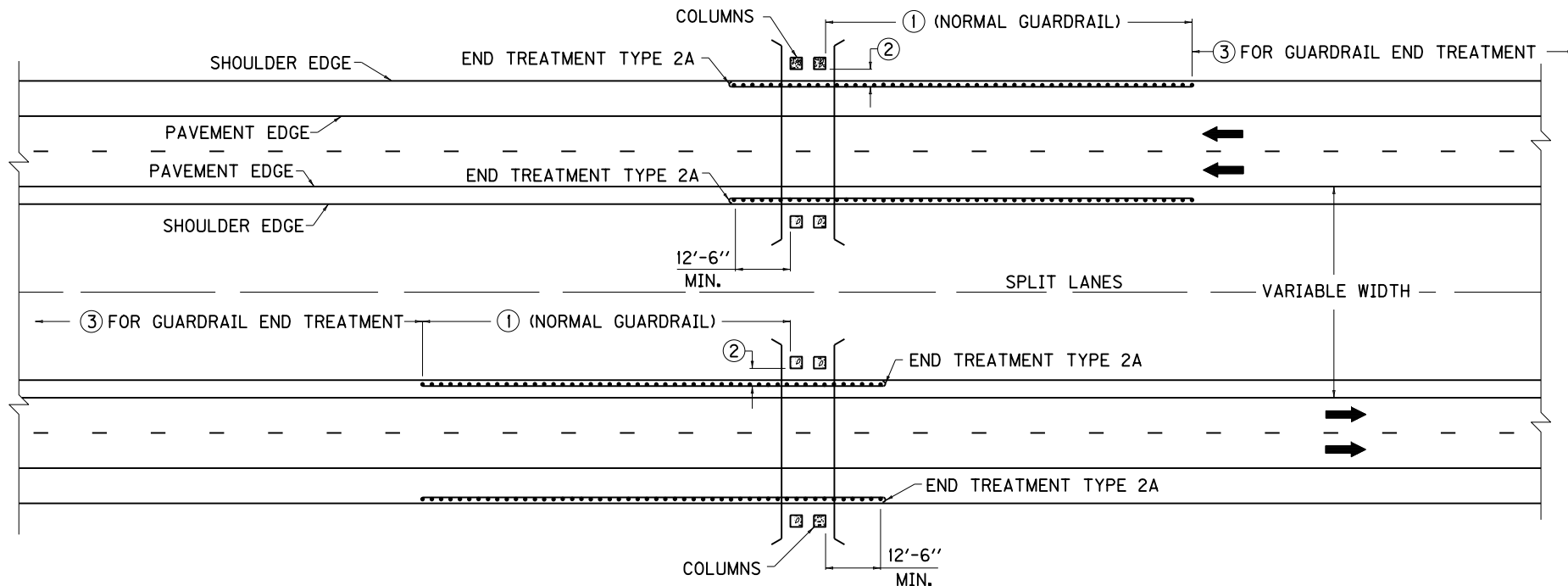
LOCATION OF GUARDRAIL WITH VARIABLE WIDTH MEDIAN
