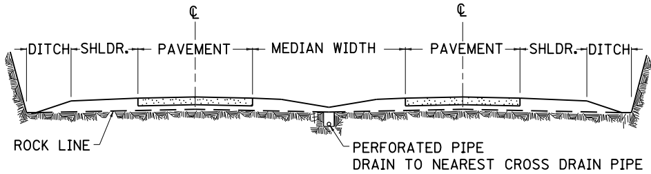
NORMAL SECTION
