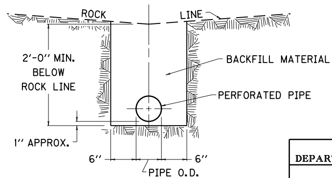
DETAIL OF PERFORATED PIPE AT LOCATIONS AS SHOWN ON THE SECTIONS
