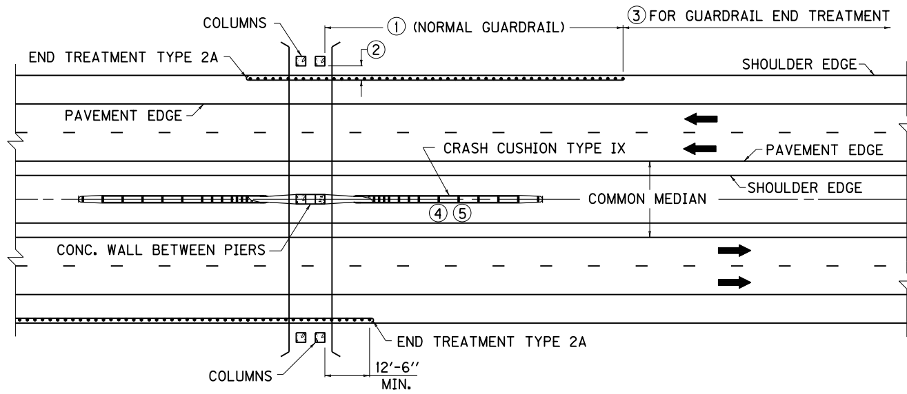
LOCATION OF GUARDRAIL WITH CONSTANT WIDTH MEDIAN
