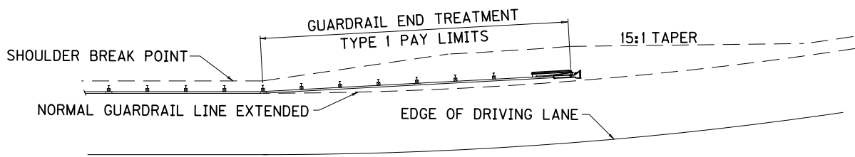
GUARDRAIL END TREATMENT TYPE 1 INSTALLED ON A CURVE ④
