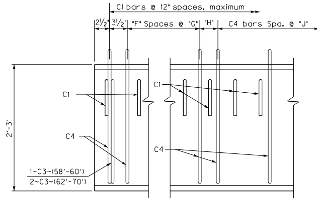
CB27 ELEVATION OF 0° SKEW
