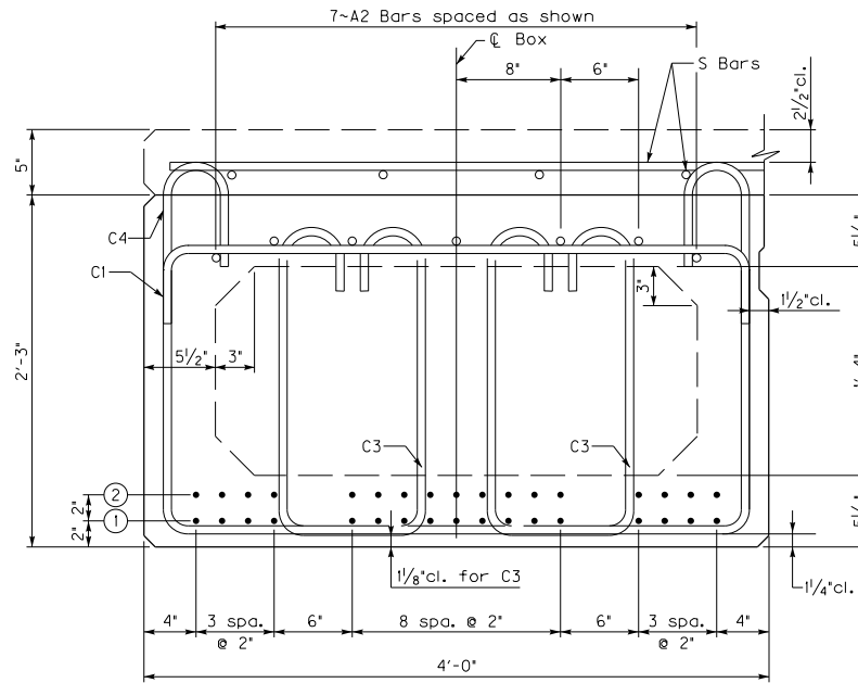
CB27 BEAM
