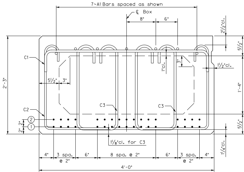
B27 BEAM
