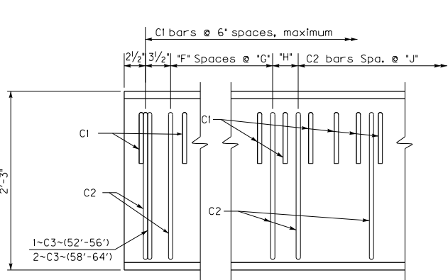
B27 ELEVATION OF 0° SKEW
