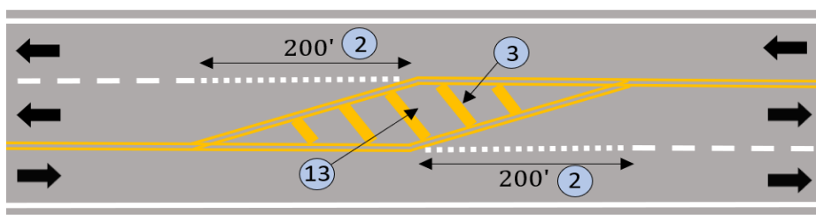
Tail to Tail Transitions
