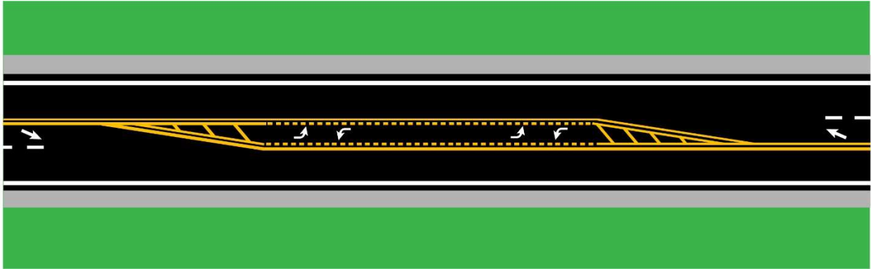
Figure 5 Schematic for Two-Way Left-Turn Lane on a 2+1 Roadway
