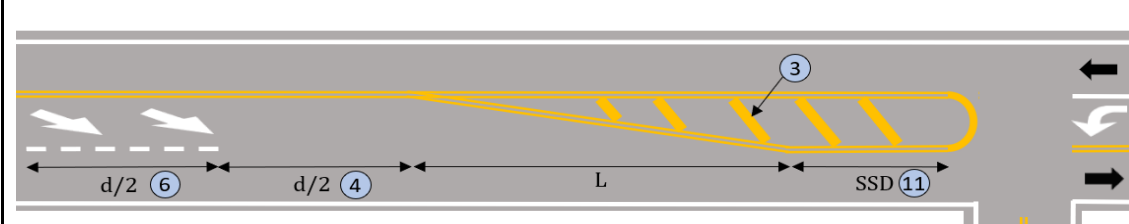
Begin Passing Lane at Intersection with Left Turn Lane
