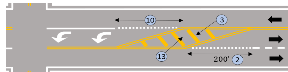
Begin Passing Lane at Intersection with Left Turn Lane
