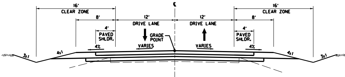
EAST AIKEN ROAD – NORMAL SECTION
