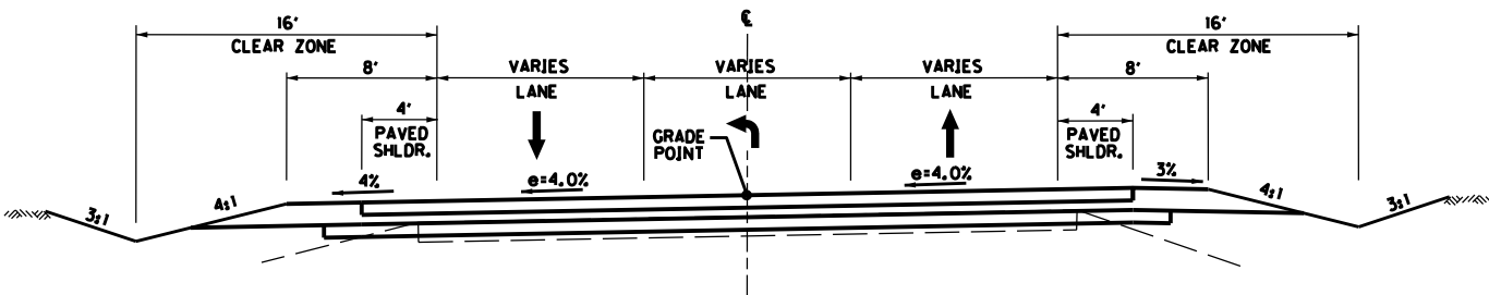
OLD HENRY ROAD – NORMAL SECTION
