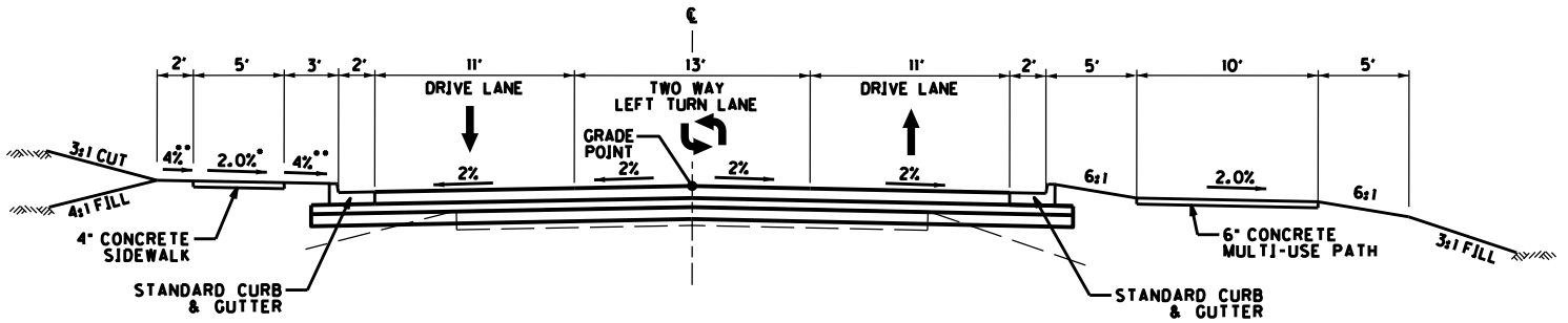
NORTH ENGLISH STATION ROAD – NORMAL SECTION
