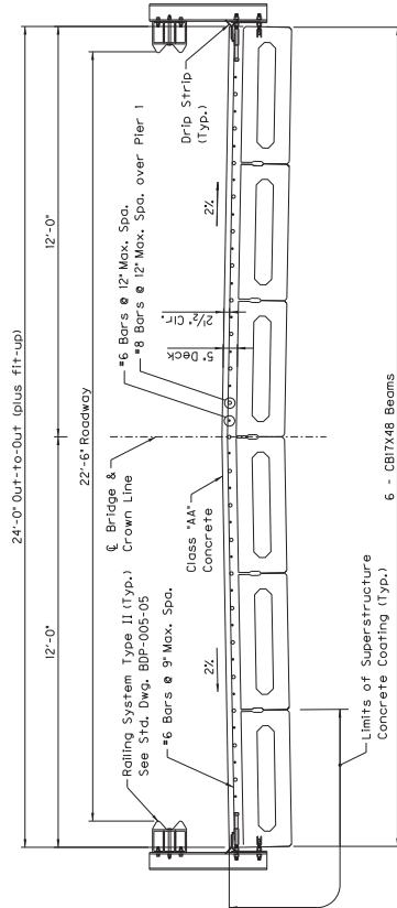
PROPOSED TYPICAL SECTION
