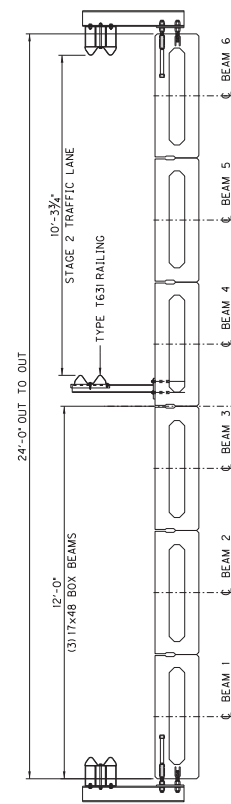
TYPICAL SECTION - STAGE 2 CONSTRUCTION
