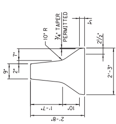
CONCRETE BARRIER WALL TYPE 9T (TEMPORARY)
