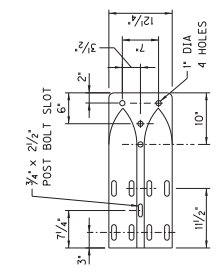
TERMINAL SECTION NO. 2
