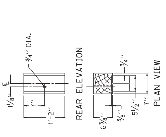
OFFSET BLOCK TYPE 6 (TIMBER OR APPROVED COMPOSITE)
