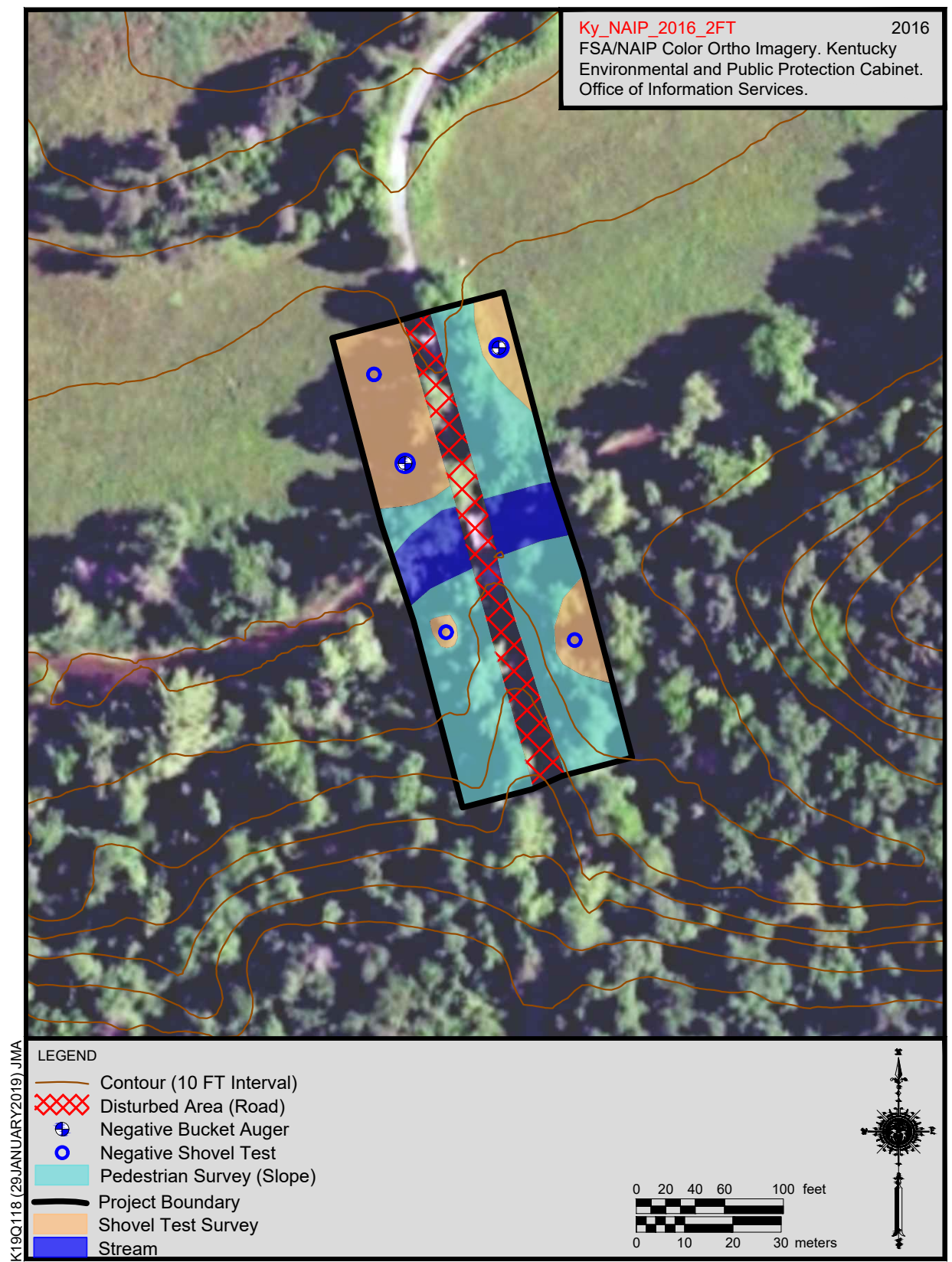
Figure 13. CR 1161 bridge (043C00011N; Item No. 4-10000.00) over Rock Creek in Grayson County showing shovel test and bucket auger locations on an aerial map.
