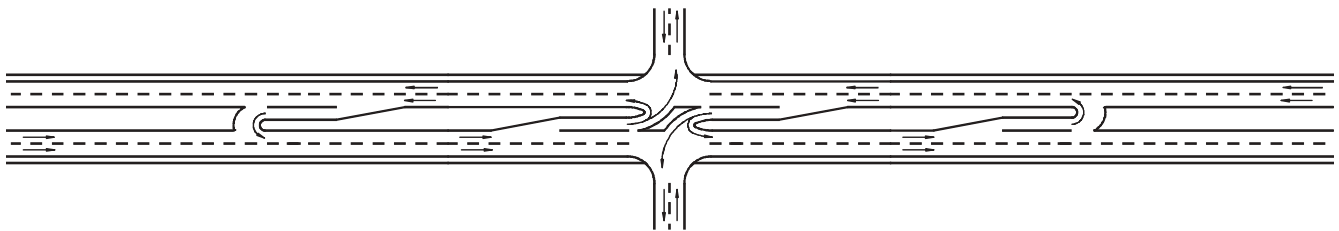
b) Directional Median Opening Four-Leg Intersection With Two Directional Midblock Median Openings (Type 2b + Type 6a + Type 2b)
