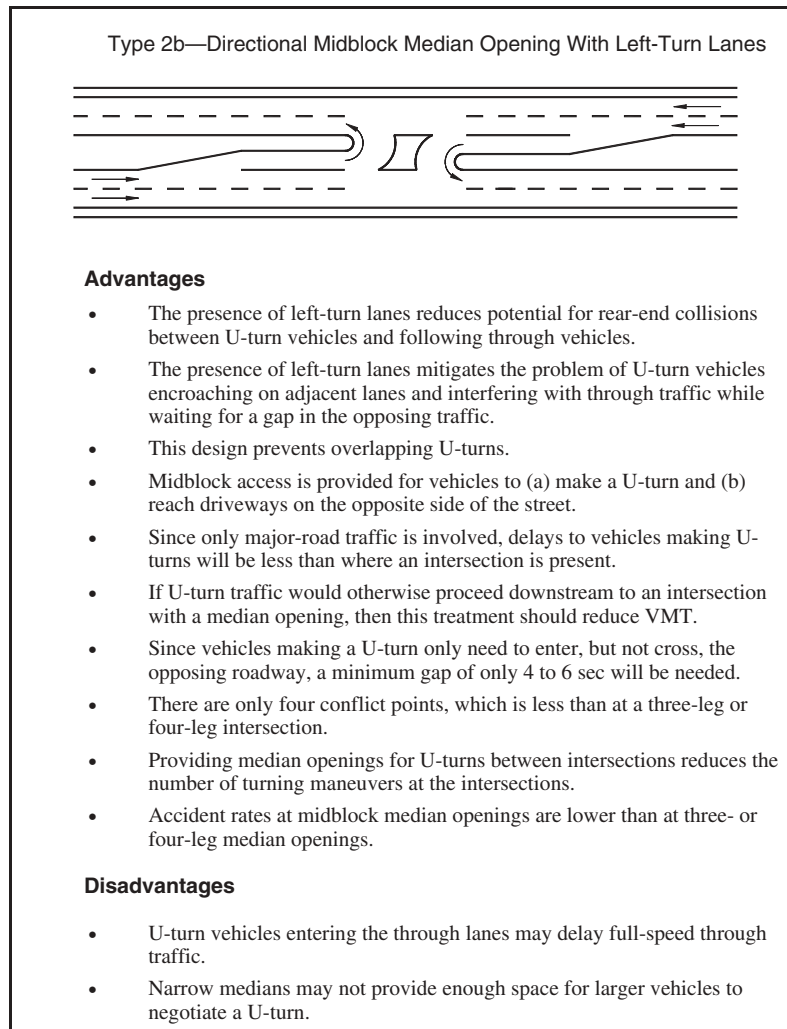
Figure C-7. Advantages and disadvantages of median opening type 2b—directional midblock median opening with left-turn lanes.
