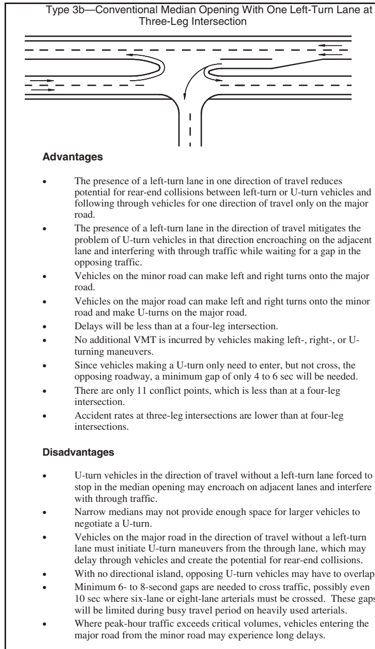
Figure 26. Advantages and disadvantages of median opening type 3b—conventional median opening with one left-turn lane at three-leg intersection.
