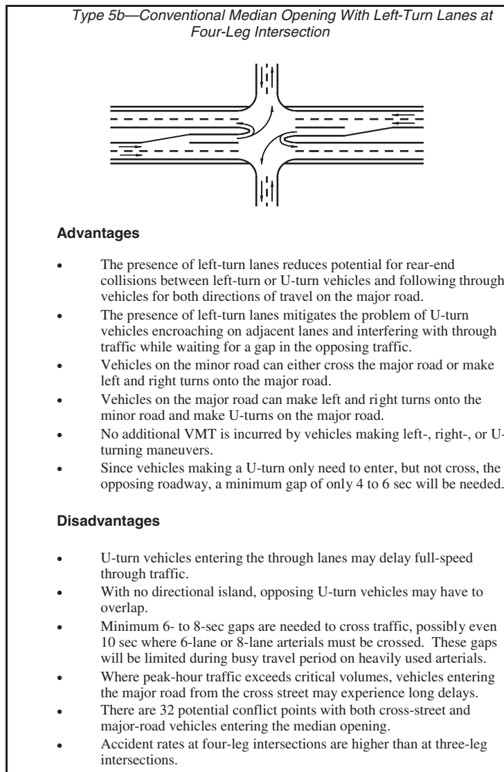
Figure 32. Advantages and disadvantages of median opening type 5b—conventional median opening with left-turn lanes at four-leg intersection.
