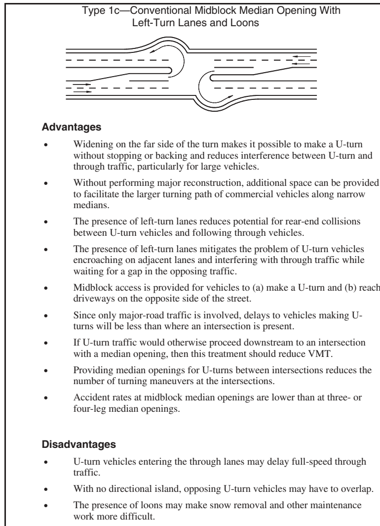
Figure C-5. Advantages and disadvantages of median opening type 1c—conventional midblock median opening with left-turn lanes and loons.
