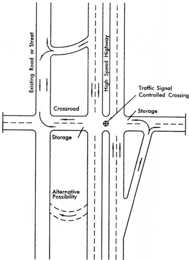
Figure 10. Special indirect left-turn designs for traffic leaving highway with narrow median (3).
