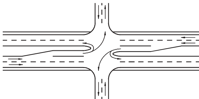
a) Conventional Median Opening at Four-Leg Intersection (Type 5b)
