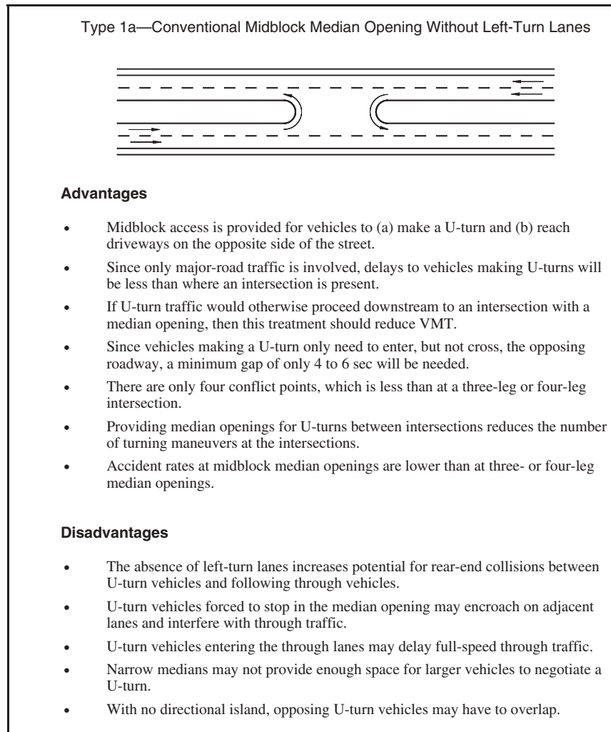
Figure C-3. Advantages and disadvantages of median opening type 1a—conventional midblock median opening without left-turn lanes.
