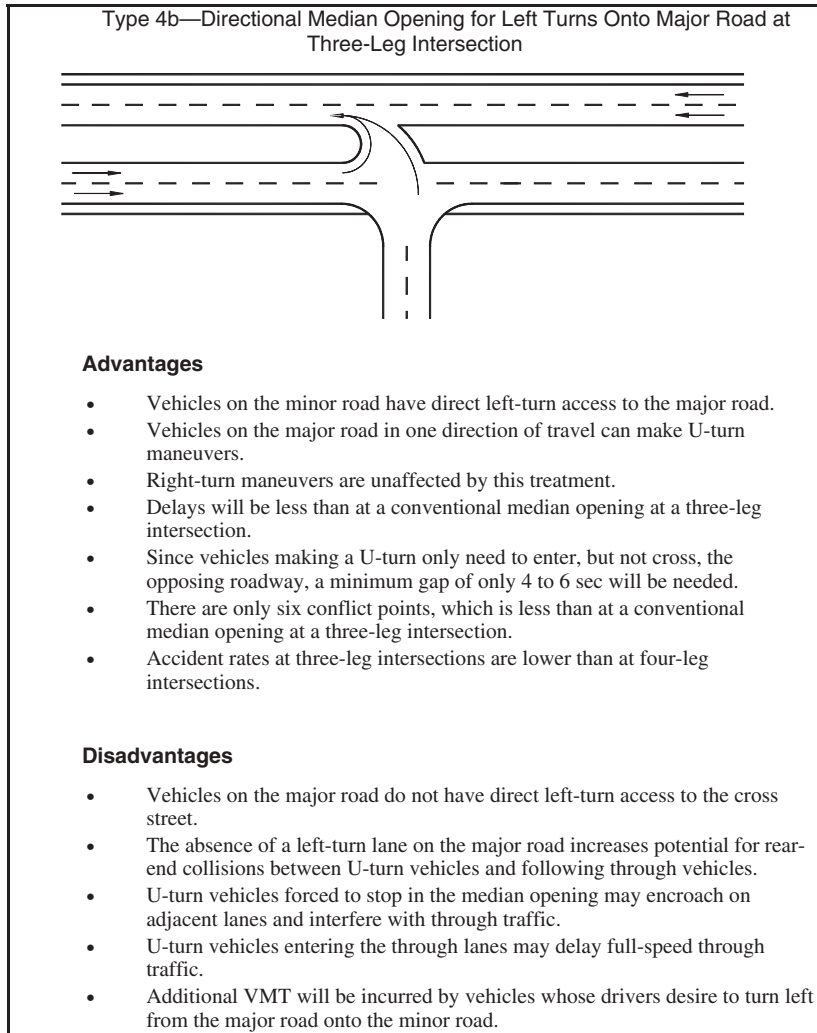
Figure C-14. Advantages and disadvantages of median opening type 4b—directional median opening for left turns onto major road at three-leg intersection.
