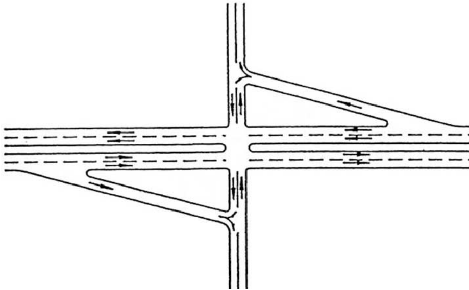
Figure 8. Jughandle-type ramp with crossroad (3).
