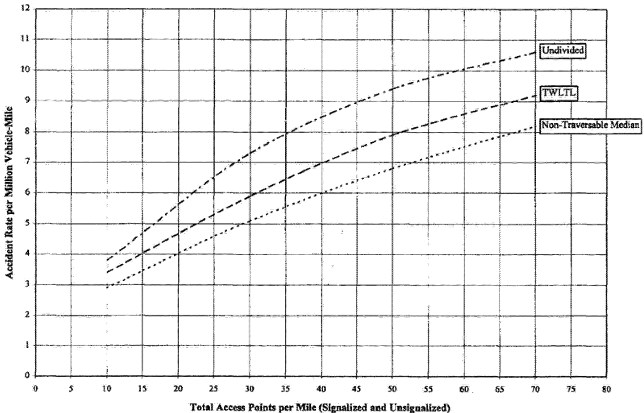
Figure C-1. Estimated accident rates by type of median-urban and suburban areas.
