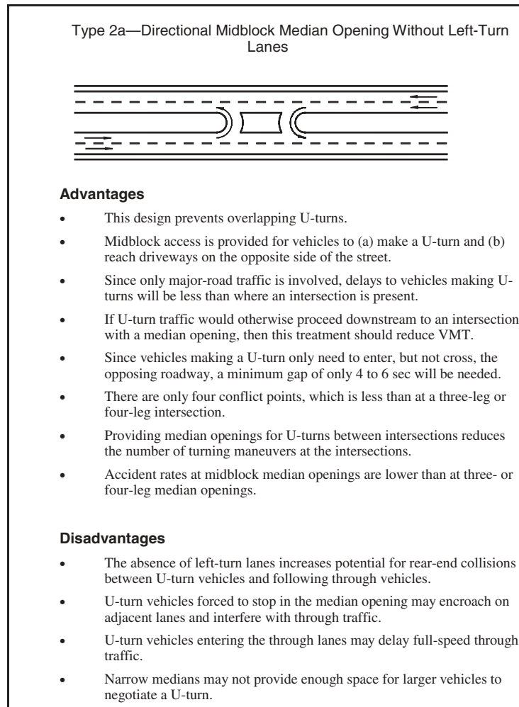
Figure 22. Advantages and disadvantages of median opening type 2a—directional midblock median opening without left-turn lanes.
