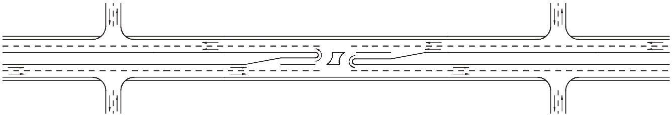
Figure 41. Combination C4—directional midblock median opening between four-leg intersections without median openings.
