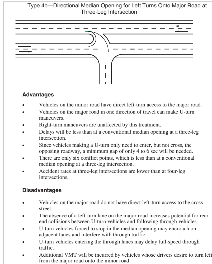
Figure 30. Advantages and disadvantages of median opening type 4b—directional median opening for left turns onto major road at three-leg intersection.
