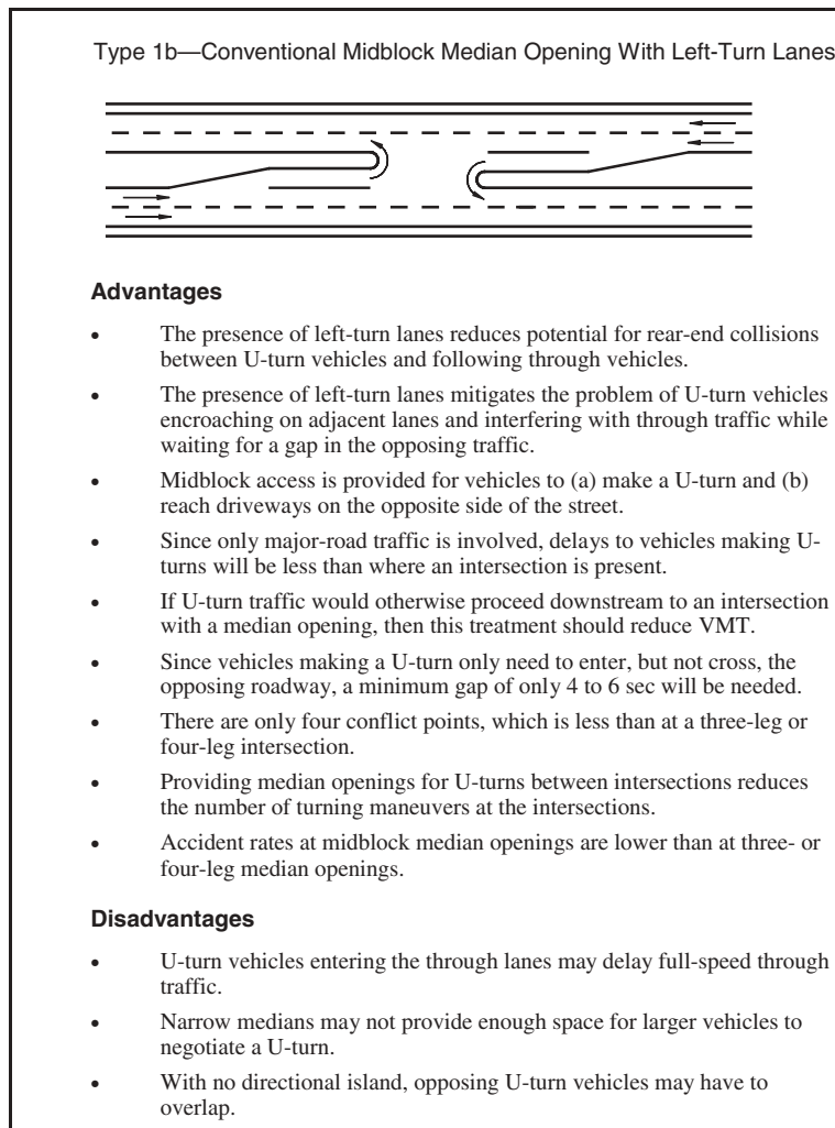
Figure 20. Advantages and disadvantages of median opening type 1b—conventional midblock median opening with left-turn lanes.
