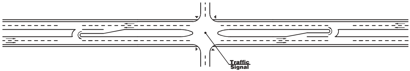
b) Signalized Four-Leg Intersection With No Turns Permitted and Two Directional Midblock Median Openings
