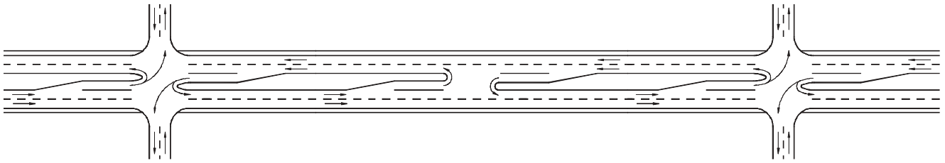
Figure 39. Combination C2—Conventional midblock median opening between four-leg intersections with conventional median openings.
