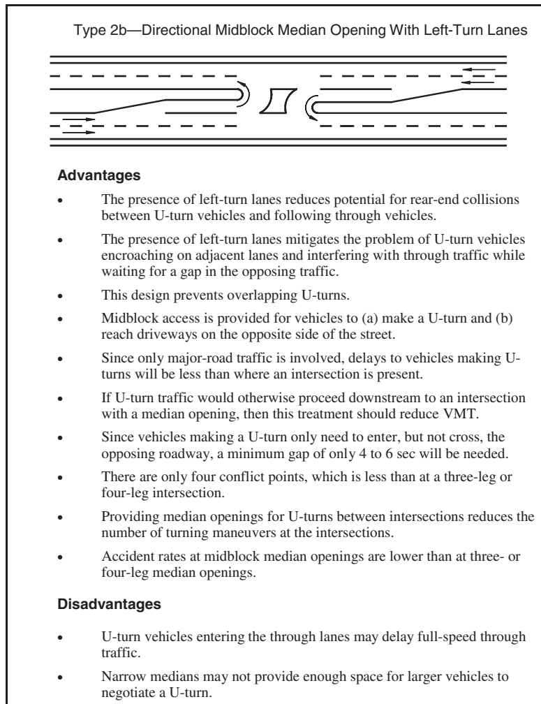
Figure 23. Advantages and disadvantages of median opening type 2b—directional midblock median opening with left-turn lanes.
