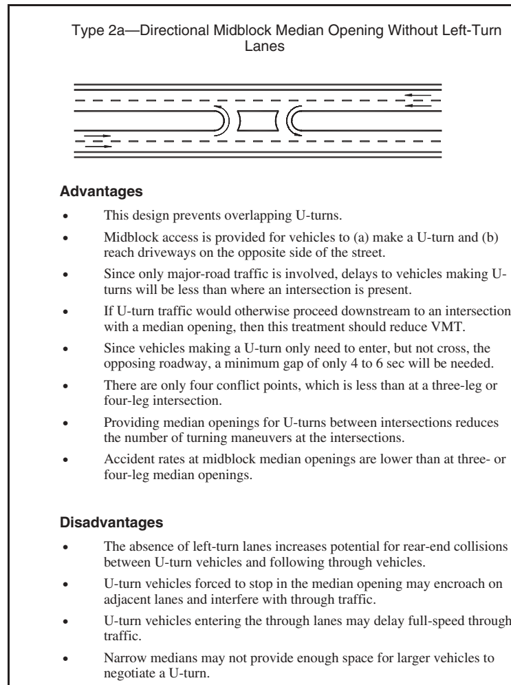
Figure C-6. Advantages and disadvantages of median opening type 2a—directional midblock median opening without left-turn lanes.
