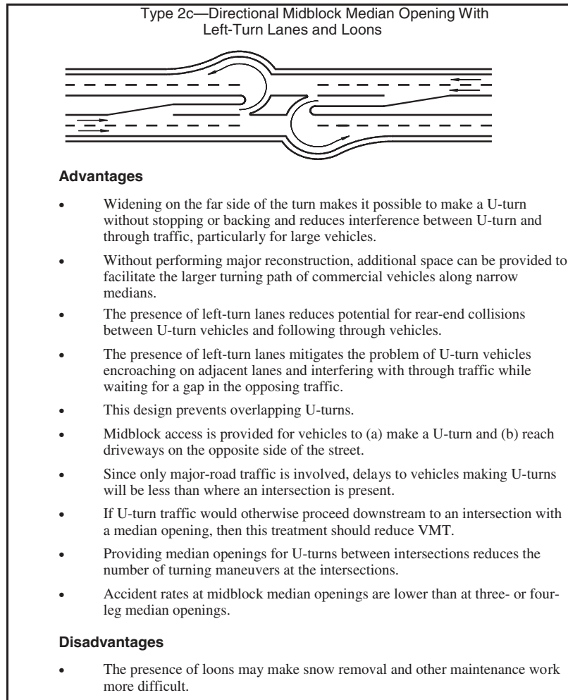
Figure 24. Advantages and disadvantages of median opening Type 2c—directional midblock median opening with left-turn lanes and loons.
