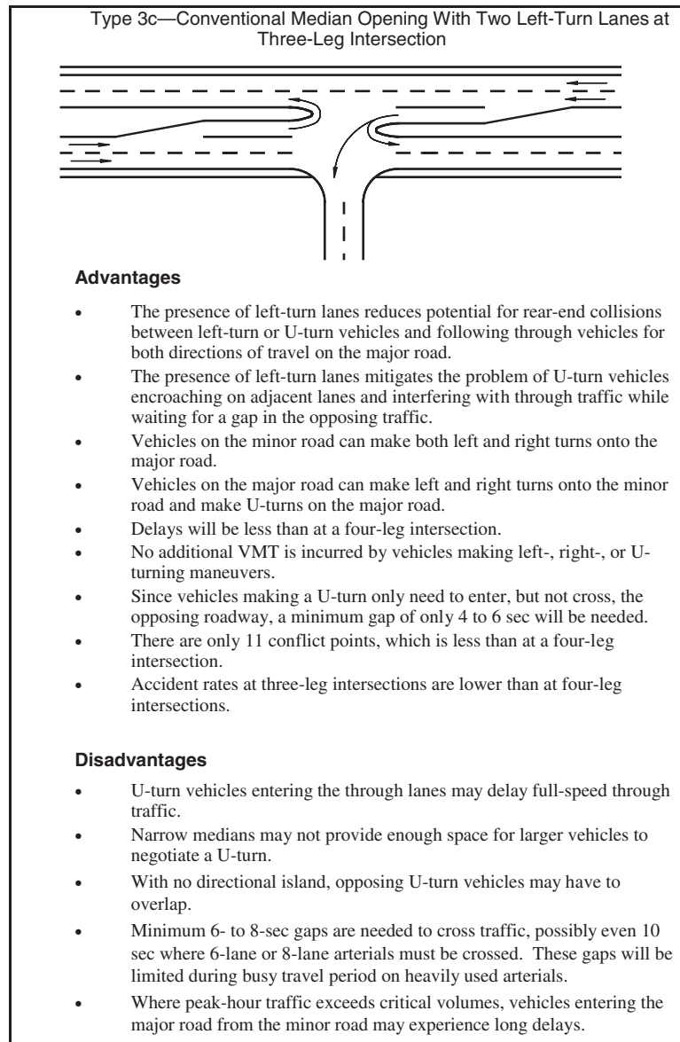
Figure 27. Advantages and disadvantages of median opening type 3c—conventional median opening with two left-turn lanes at three-leg intersection.
