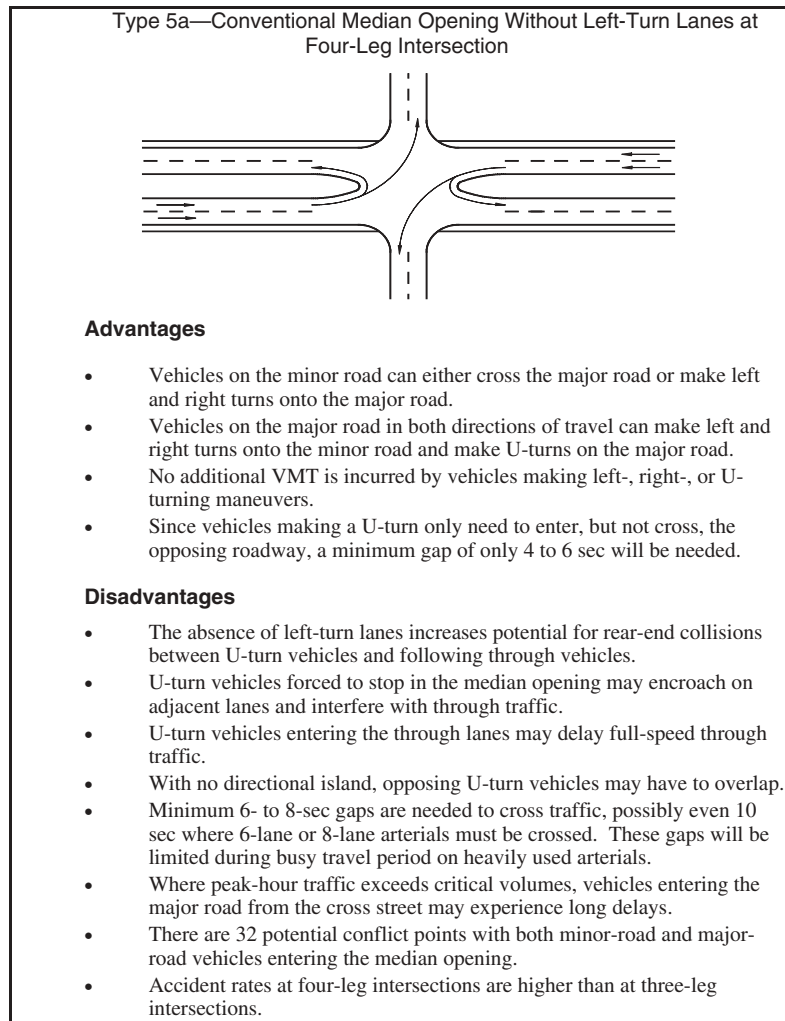
Figure C-15. Advantages and disadvantages of median opening type 5a—conventional median opening without left-turn lanes at four-leg intersection.
