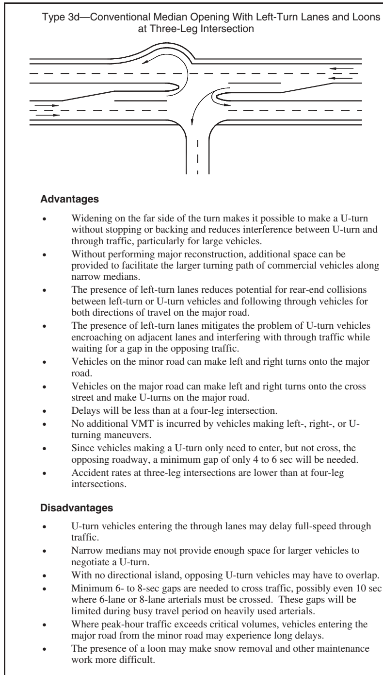
Figure C-12. Advantages and disadvantages of median opening type 3d—conventional median opening with left-turn lanes and loons at three-leg intersection.
