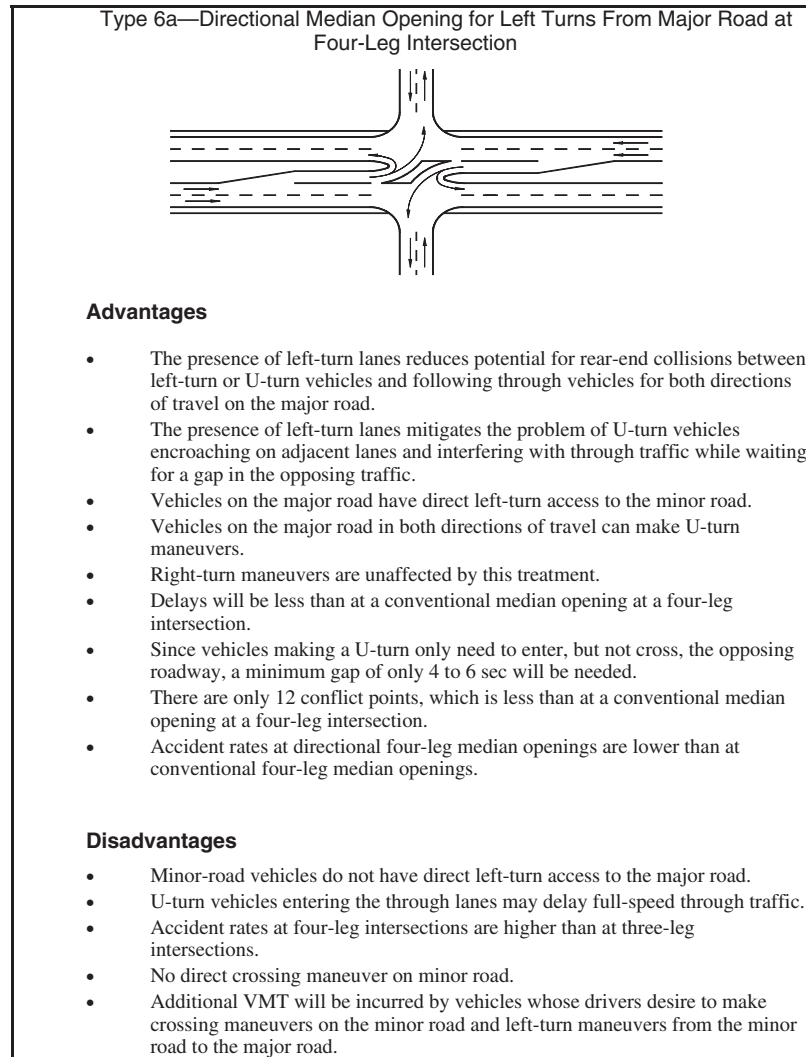
Figure C-17. Advantages and disadvantages of median opening type 6a—directional median opening for left turns from major road at four-leg intersection.
