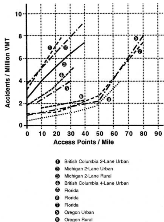
Figure 12. Composite accident rates as a function of access point density (4).
