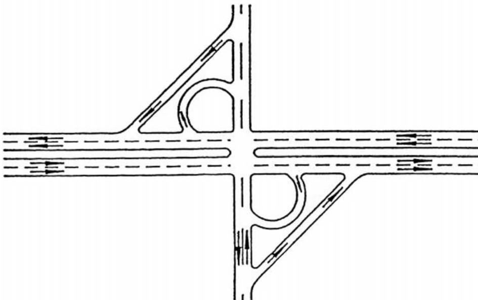
Figure 9. At-grade loop (surface loop) with crossroad (3).
