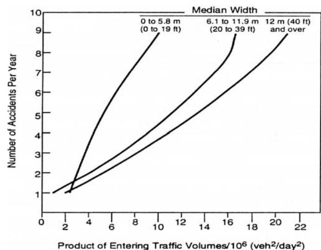
Figure 4. Variation of annual accident frequency at divided highway intersections as a function of median width and exposure index (the product of the ADTs of the intersecting roadways) (10).
