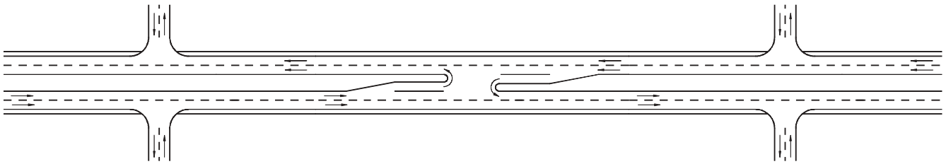
Figure 43. Combination C6—conventional midblock median opening between four-leg intersections without median openings.
