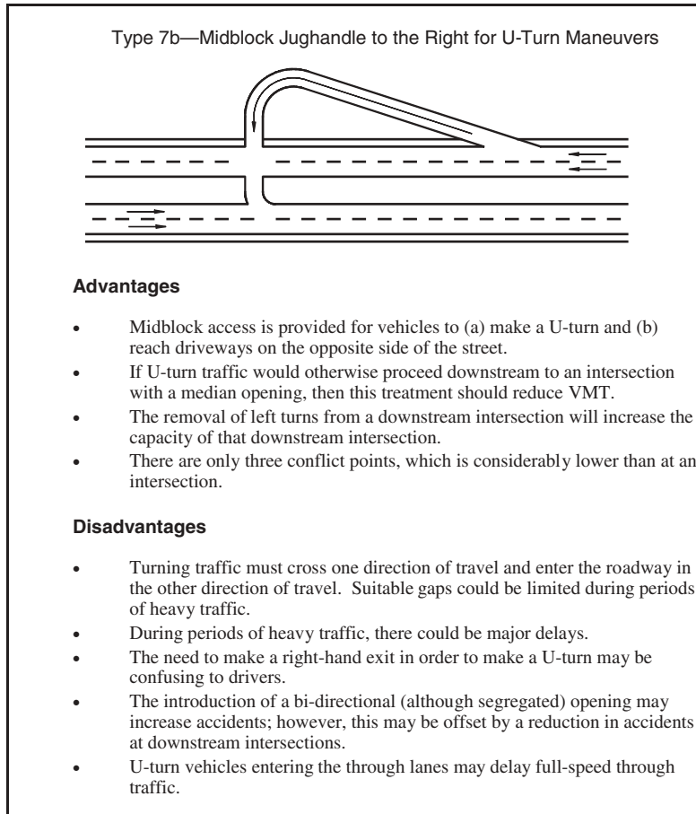
Figure 35. Advantages and disadvantages of median opening type 7b—midblock jughandle to the right for U-turn maneuvers.
