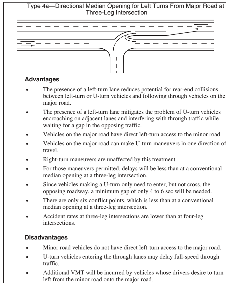
Figure C-13. Advantages and disadvantages of median opening type 4a—directional median opening for left turns from major road at three-leg intersection.
