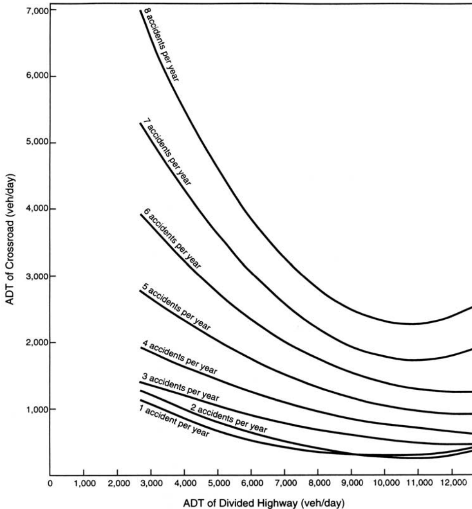
Figure 2. Average number of accidents per year related to traffic volume at divided highway intersections (10).
