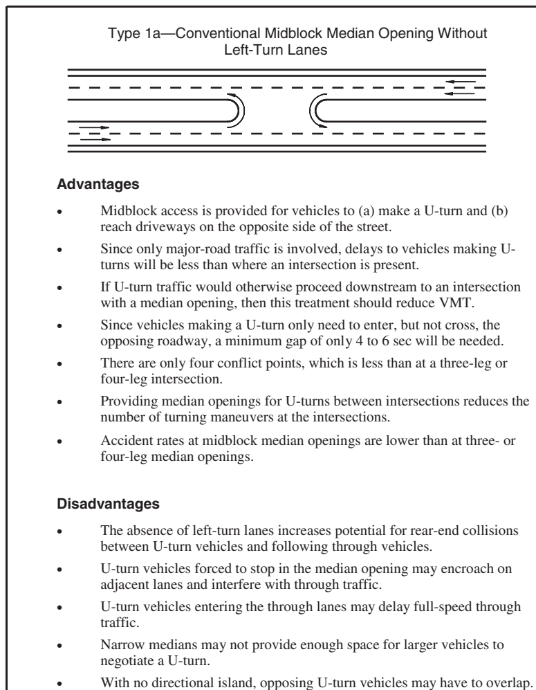
Figure 19. Advantages and disadvantages of median opening type 1a—conventional midblock median opening without left-turn lanes.
