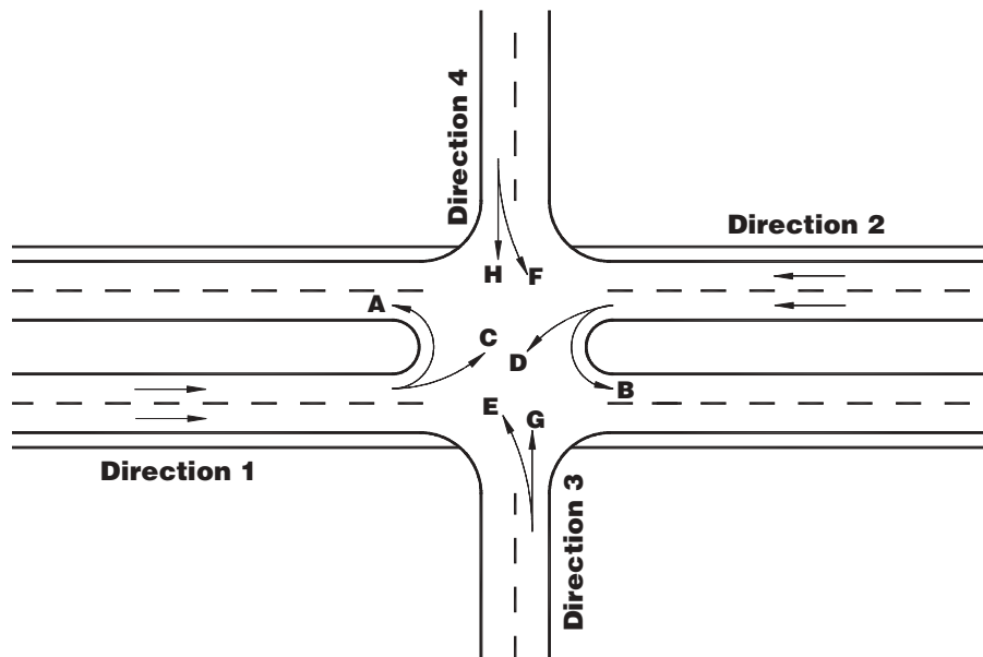
Figure C-20. Turning movements at a four-leg intersection.
