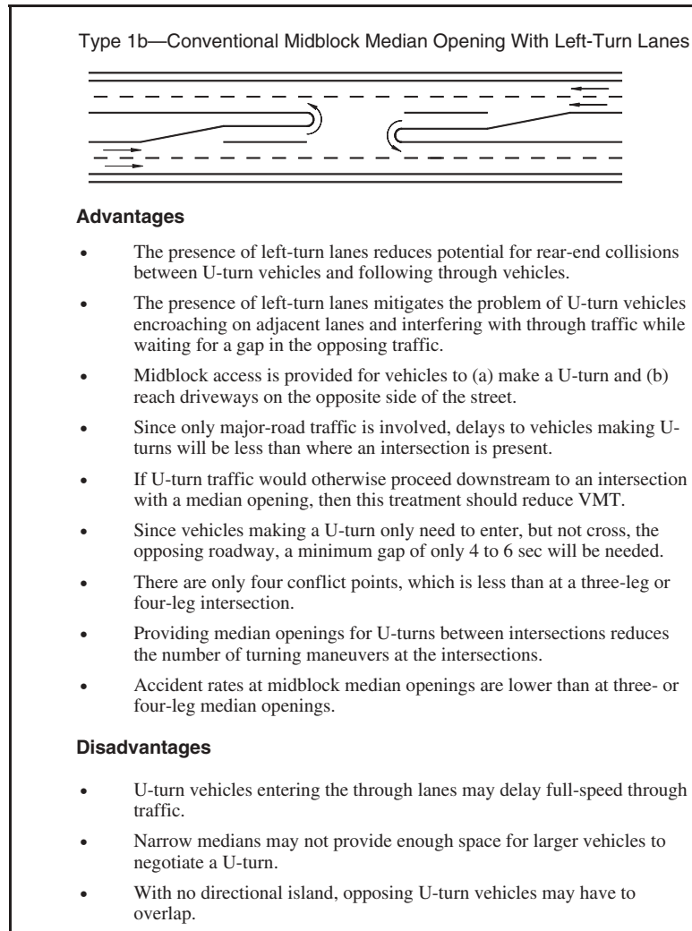
Figure C-4. Advantages and disadvantages of median opening type 1b—conventional midblock median opening with left-turn lanes.
