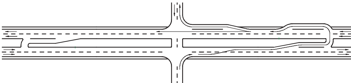
Figure 7. Typical loon design at a directional median opening (55, 56).
