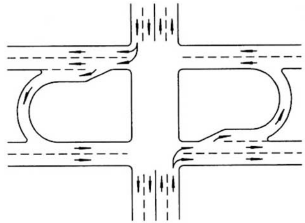
Figure 11. Indirect left turn through a crossover (3).
