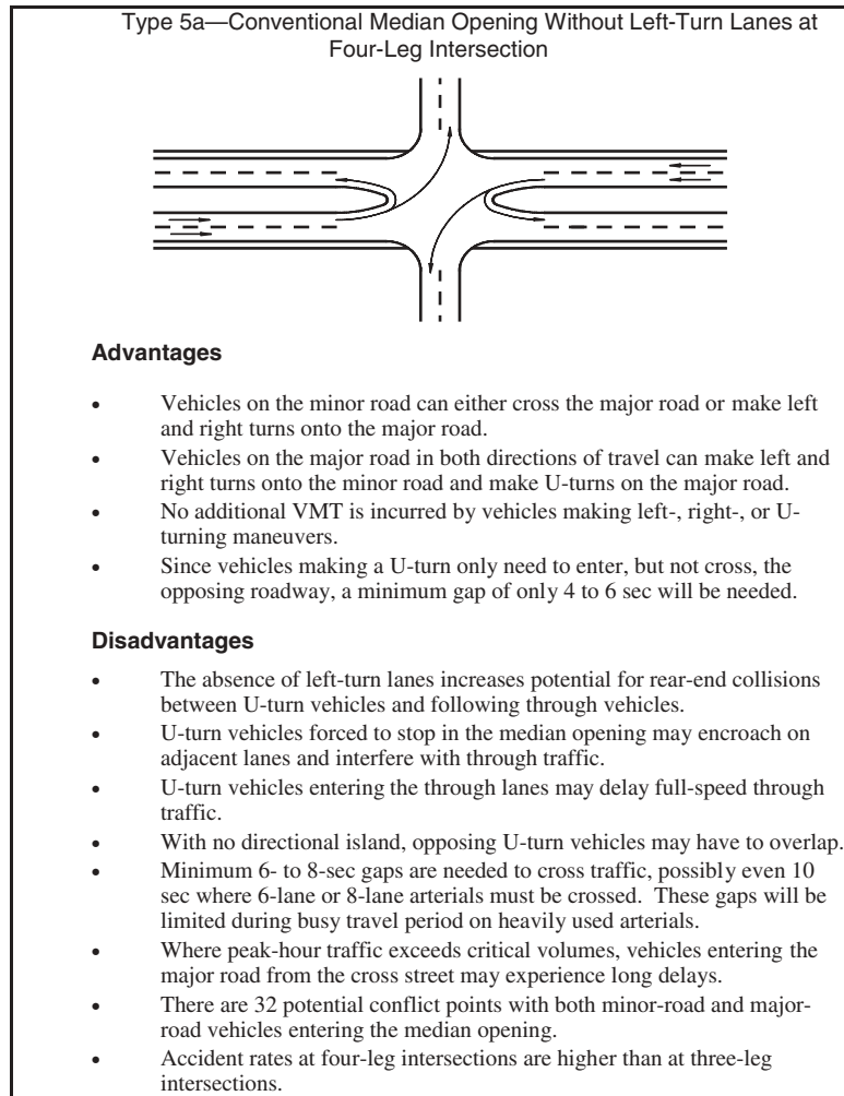
Figure 31. Advantages and disadvantages of median opening Type 5a—conventional median opening without left-turn lanes at four-leg intersection.
