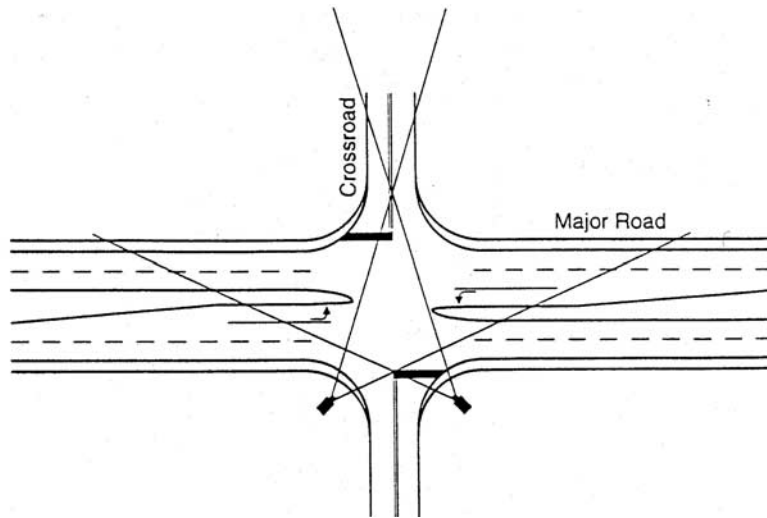
Figure 46. Typical data collection setup using video cameras (8).
