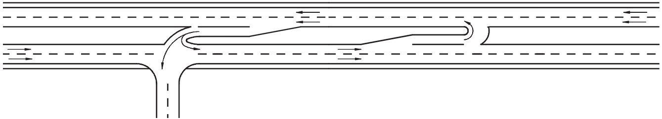
b) Directional Median Opening For Left Turns From Major Road at Three-Leg Intersection With Directional Midblock Median Opening (Type 4a + Type 2b)
