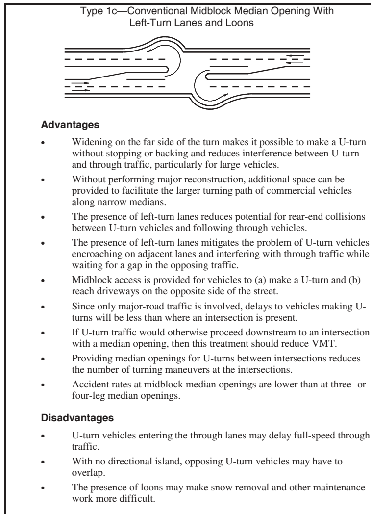
Figure 21. Advantages and disadvantages of median opening type 1c—conventional midblock median opening with left-turn lanes and loons.
