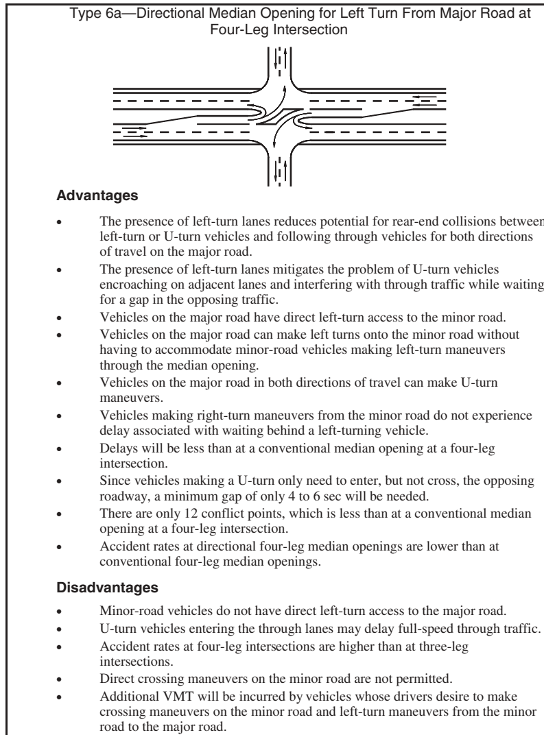
Figure 33. Advantages and disadvantages of median opening type 6a—directional median opening for left turn from major road at four-leg intersection.
