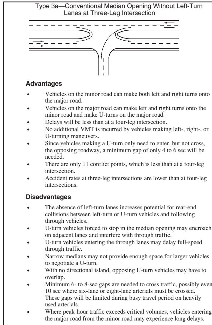
Figure C-9. Advantages and disadvantages of median opening type 3a—conventional median opening without left-turn lanes at three-leg intersection.
