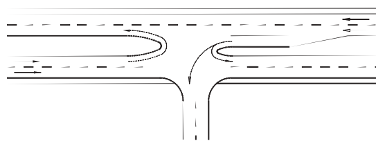
a) Conventional Median Opening at Three-Leg Intersection (Type 3b)
