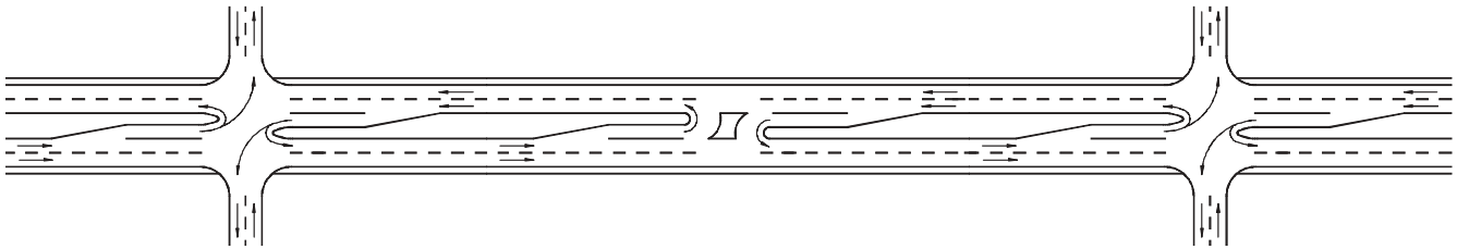
Figure 40. Combination C3—Directional midblock median opening between four-leg intersections with conventional median openings.
