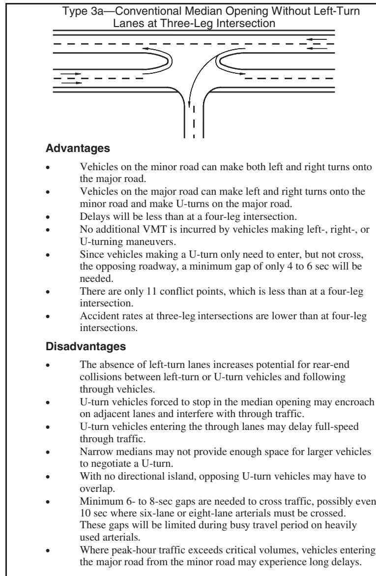
Figure 25. Advantages and disadvantages of median opening type 3a—conventional median opening without left-turn lanes at three-leg intersection.
