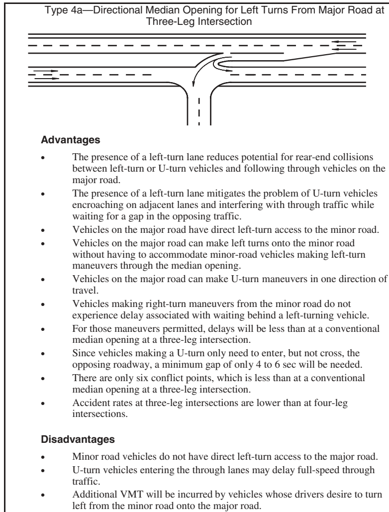
Figure 29. Advantages and disadvantages of median opening type 4a—directional median opening for left turns from major road at three-leg intersection.
