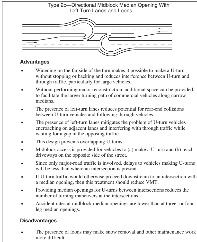
Figure C-8. Advantages and disadvantages of median opening Type 2c—directional midblock median opening with left-turn lanes and loops.
