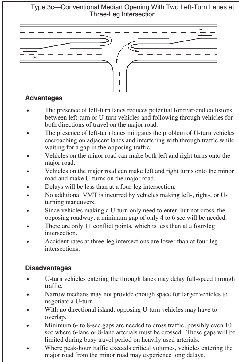
Figure C-11. Advantages and disadvantages of median opening type 3c—conventional median opening with two left-turn lanes at three-leg intersection.
