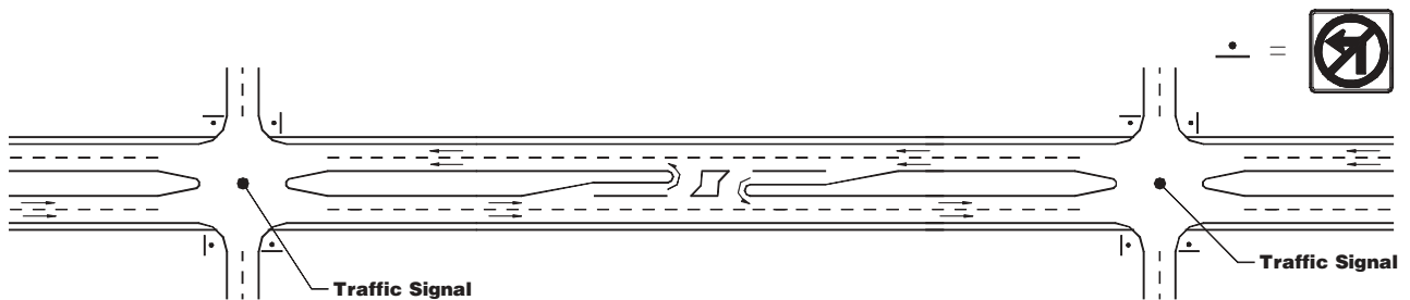
Figure 45. Combination C8—directional midblock median opening between four-leg signalized intersections with conventional median openings but all left-turning movements prohibited.
