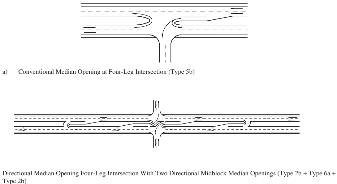
Figure C-22. Conventional and directional median openings at four-leg intersection.
