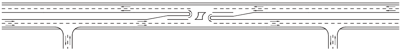
Figure 42. Combination C5—directional midblock median opening between three-leg intersections without median openings.
