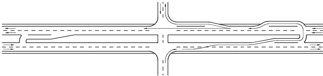
Figure C-19. Typical loon design at a directional median opening (55, 56).
