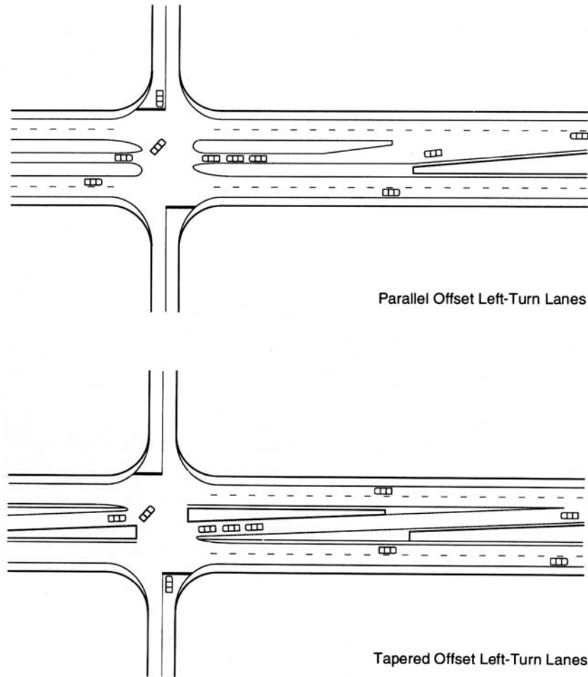
Figure 5. Examples of offset left-turn lanes (3).
