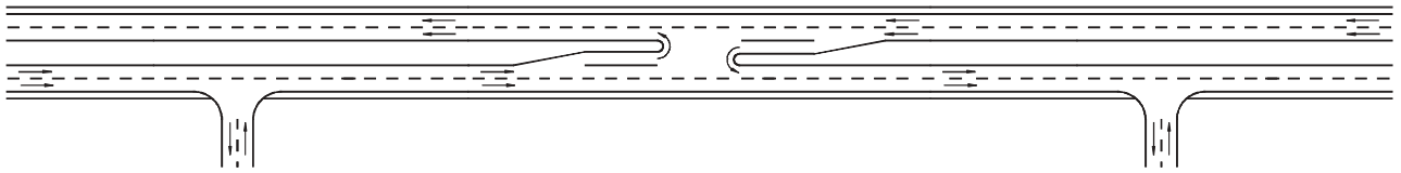
Figure 44. Combination C7—conventional midblock median opening between three-leg intersections without median openings.
