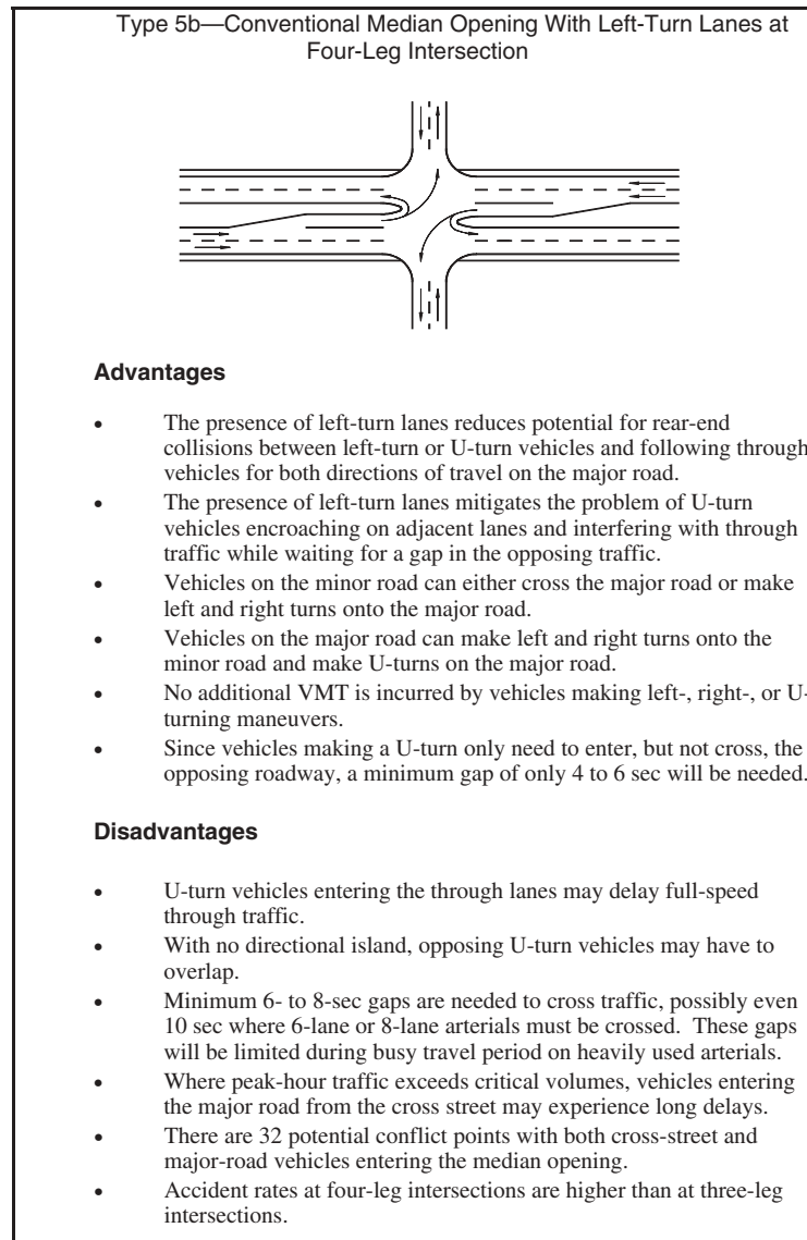
Figure C-16. Advantages and disadvantages of median opening type 5b—conventional median opening with left-turn lanes at four-leg intersection.
