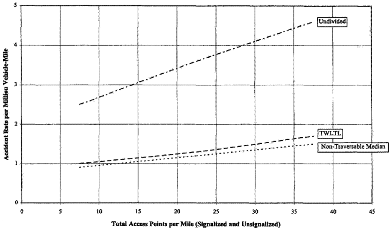
Figure C-2. Estimated accident rates by type of median-rural areas (4).
