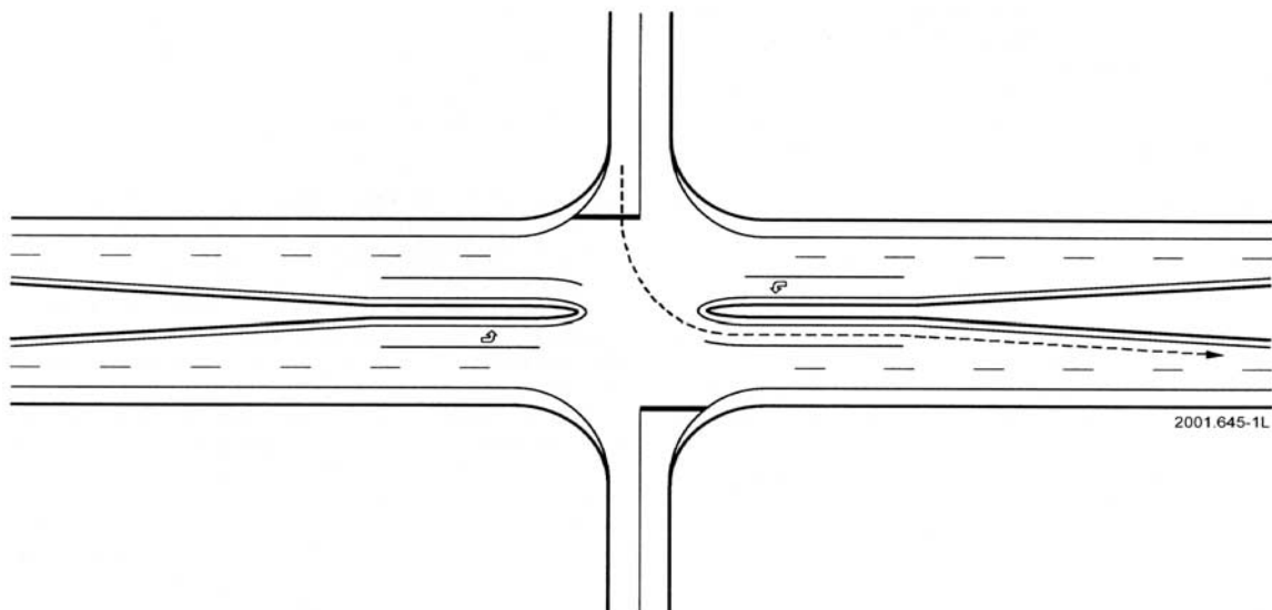
Figure 6. Typical divided highway intersection with median acceleration lanes (7).
