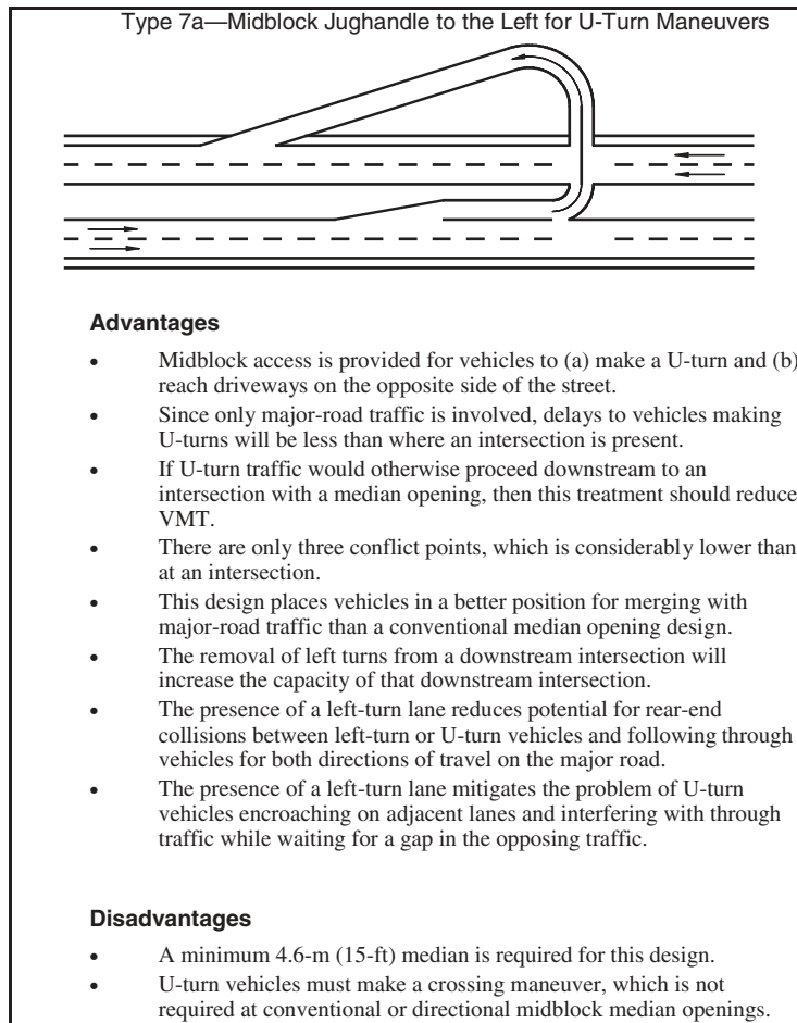
Figure 34. Advantages and disadvantages of median opening type 7a—midblock jughandle to the left for U-turn maneuvers.
