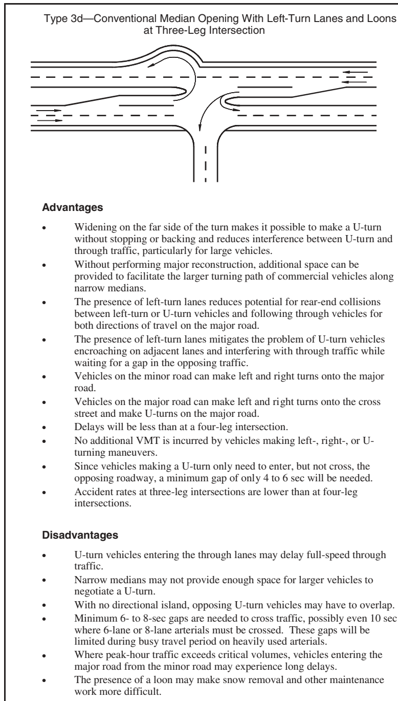
Figure 28. Advantages and disadvantages of median opening type 3d—conventional median opening with left-turn lanes and loons at three-leg intersection.
