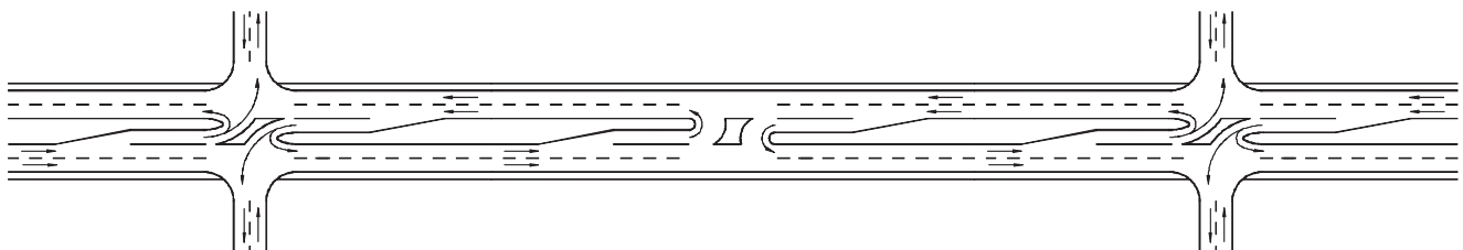
Figure 38. Combination C1—directional midblock median opening between four-leg intersections with directional median openings.
