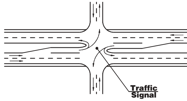
a) Conventional Median Opening at Signalized Four-Leg Intersection
