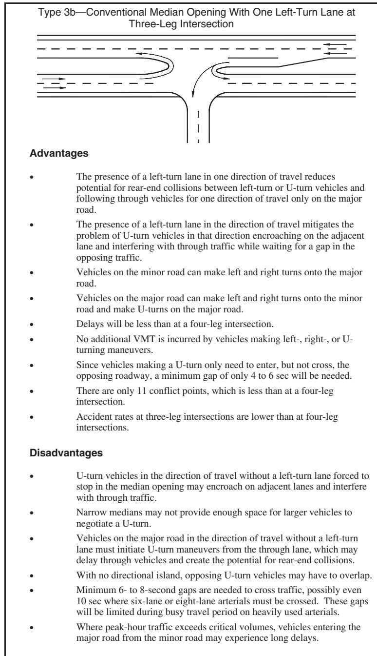
Figure C-10. Advantages and disadvantages of median opening type 3b—conventional median opening with one left-turn lane at three-leg intersection.
