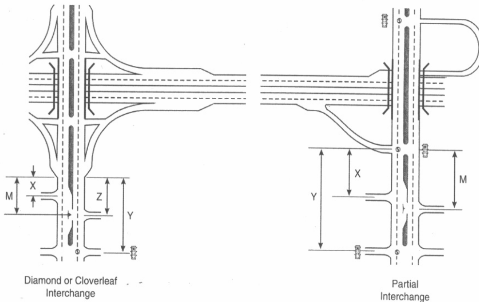
Figure 9-2 Freeway Interchange Areas with Multi-lane Crossroads
