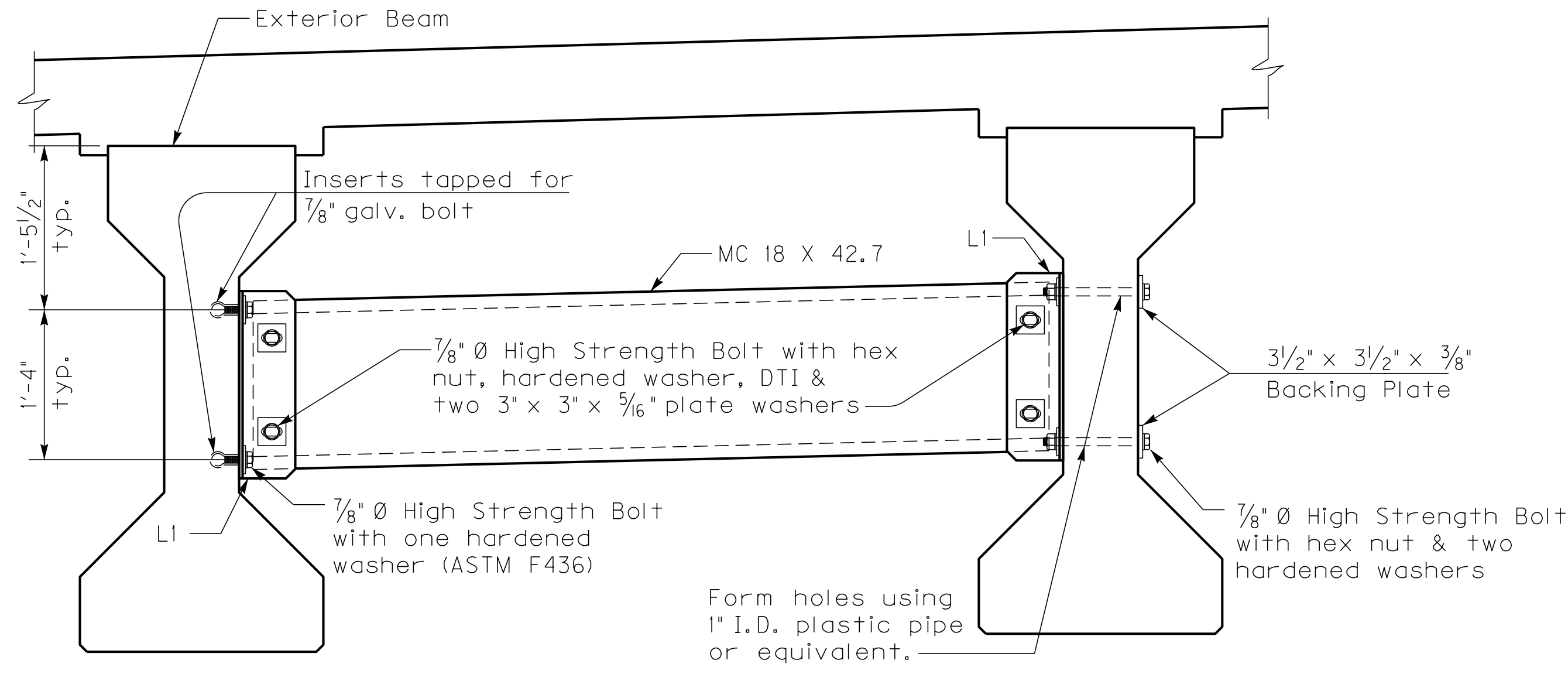
INTERMEDIATE DIAPHRAGM ~Typical for Skewed PCI, Type 4 Beams~
