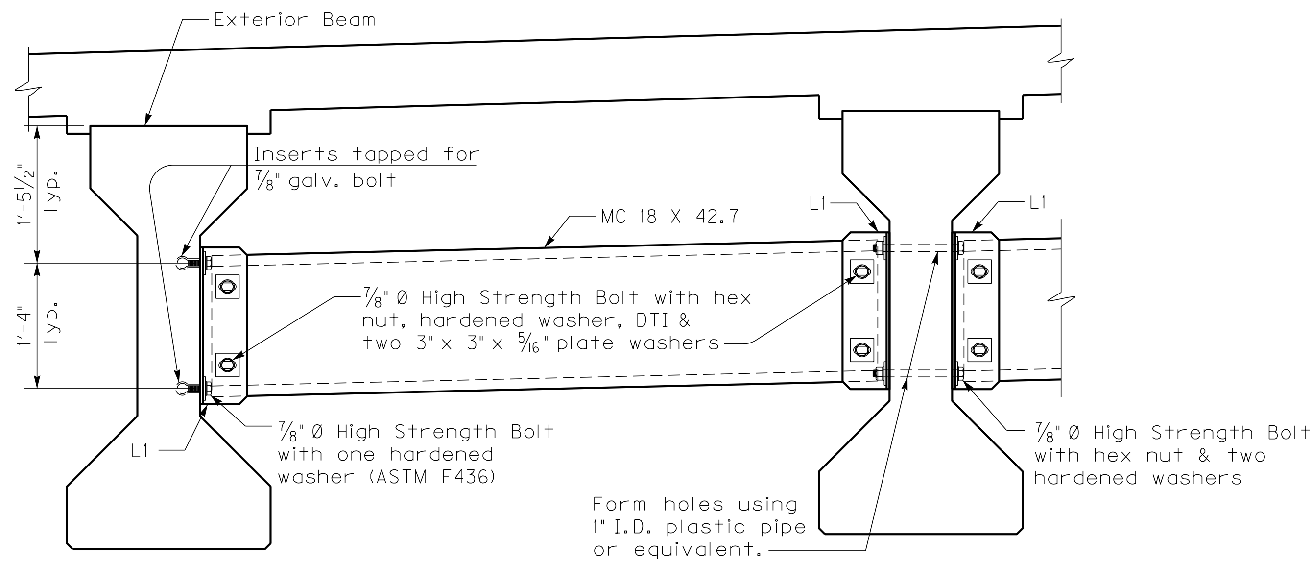
INTERMEDIATE DIAPHRAGM ~Typical for 0° Skew PCI, Type 4 Beams~
