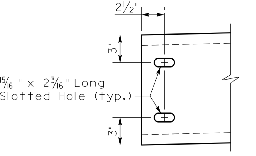
CHANNEL END
