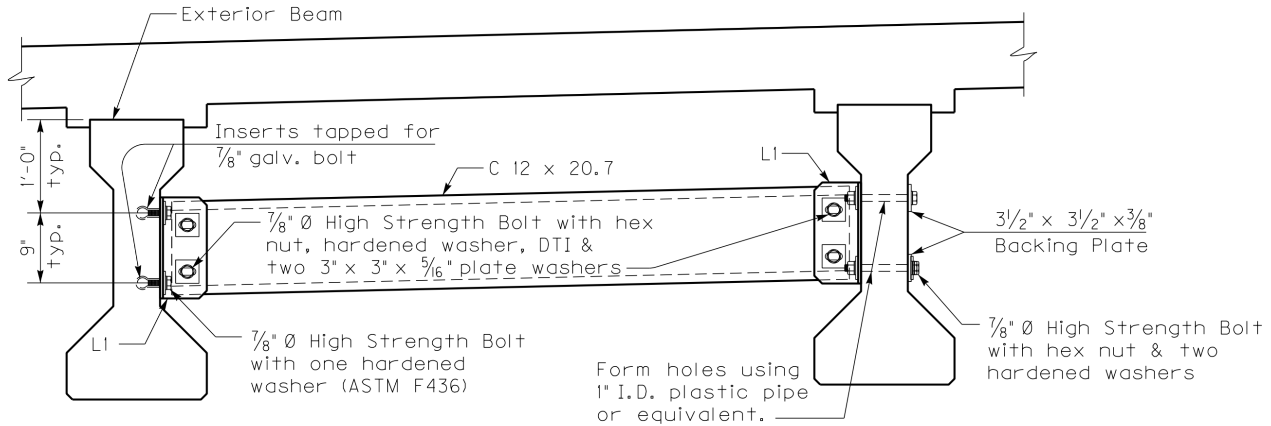
INTERMEDIATE DIAPHRAGM ~Typical for Skewed PCI, Type 2 Beams~
