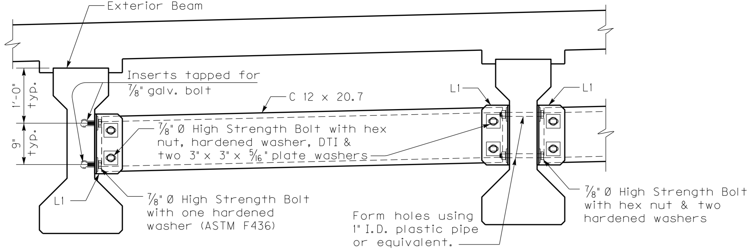
INTERMEDIATE DIAPHRAGM ~Typical for 0° Skew PCI, Type 2 Beams~
