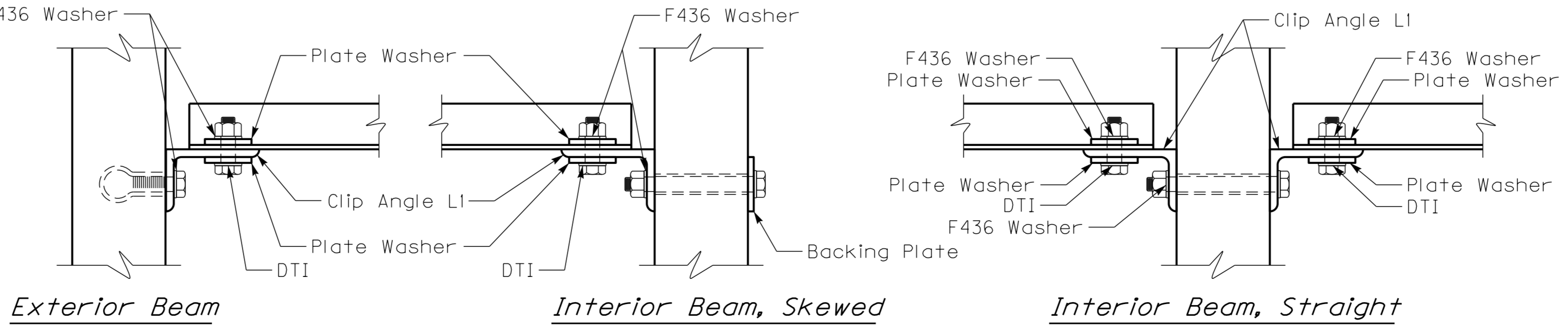
CONNECTION DETAILS
