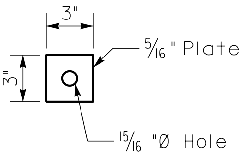
PLATE WASHER
