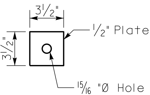
FILLER PLATE
