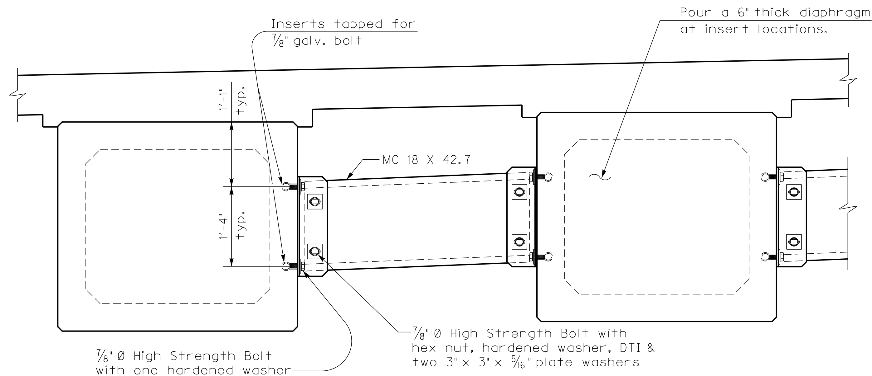
INTERMEDIATE DIAPHRAGM ~Typical for SB-42 Beams~
