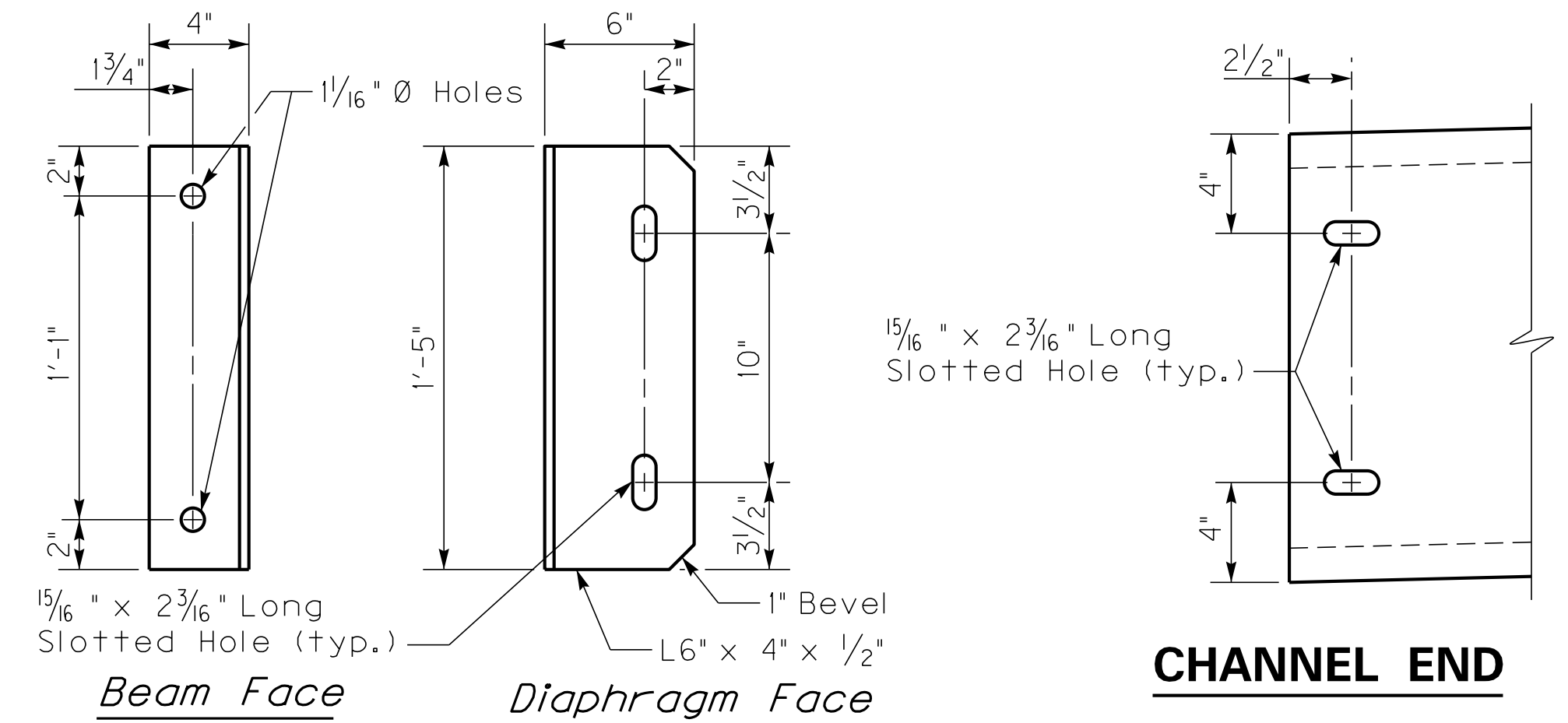
CLIP ANGLE
