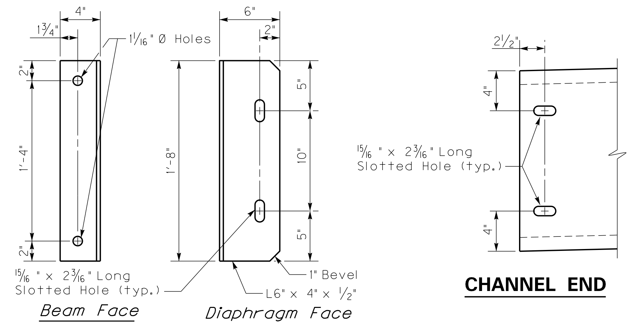
CLIP ANGLE
