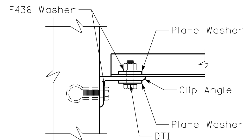
CONNECTION DETAILS
