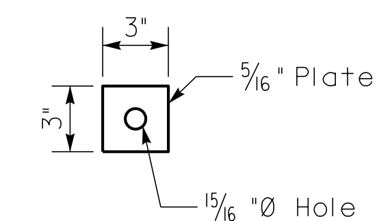
PLATE WASHER
