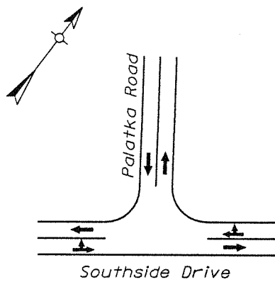
LANE DIAGRAM (EXISTING INTERSECTION)
