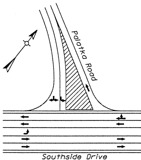
LANE DIAGRAM (PROPOSED INTERSECTION)
