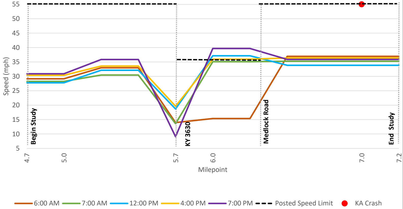
KY 578 Southbound 50th Percentile Truck Speed
