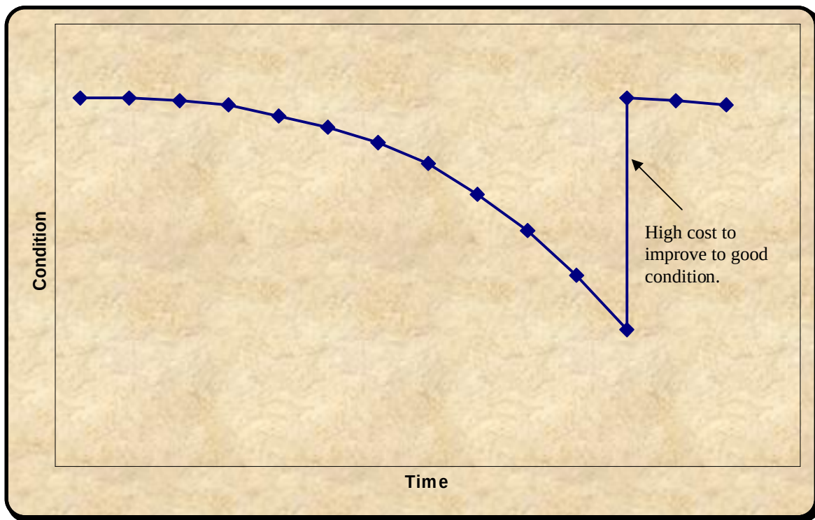
Figure 11: Pavement Condition with “Worst-First” Strategy
