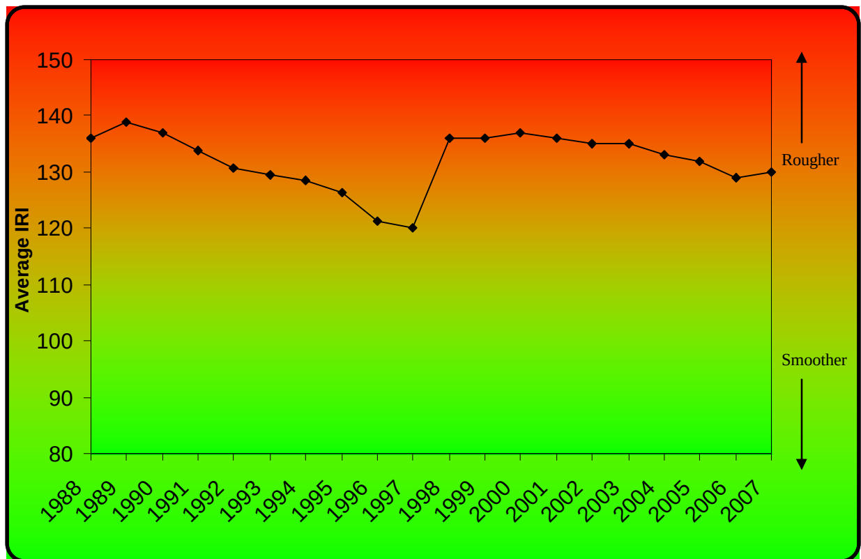
Figure 7: Average Statewide Roughness for RS Roads Since 1988
