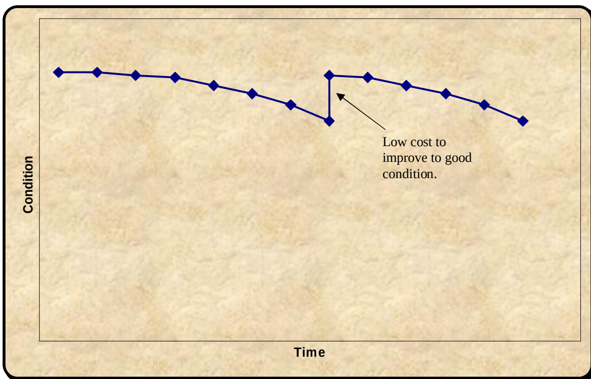
Figure 12: Pavement Condition with Preventive Maintenance Strategy
