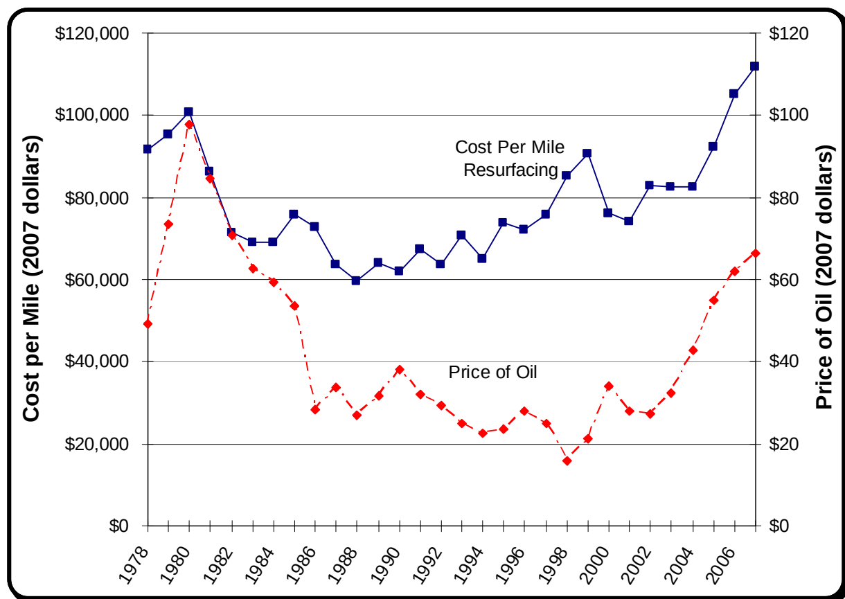
Figure 10: MP Resurfacing Costs vs. Price of Oil
