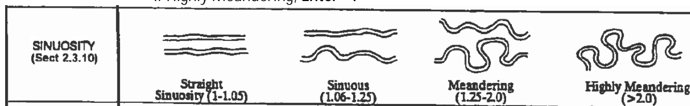
Figure 5: Sinuosity
