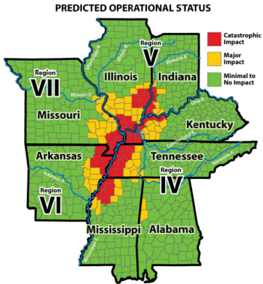
Figure 2: The eight CUSEC member states and the four FEMA regions of the New Madrid Seismic Zone
