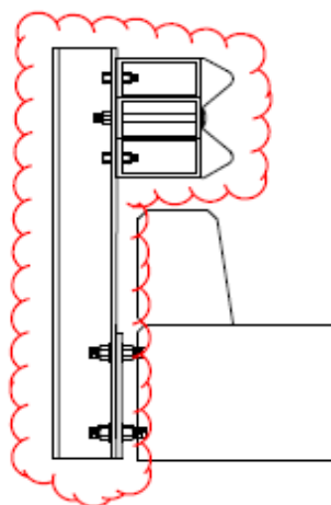
Railing System Type II with Brush Curb
