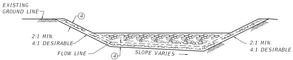
SECTION B-B
