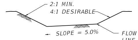
SECTION G-G
