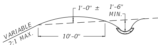
TYPICAL PAVED DITCH (INTERCEPTOR DITCH)
