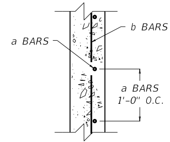
SECTION A-A CURB BOX INLET TYPE A AND CURB BOX INLET TYPE B
