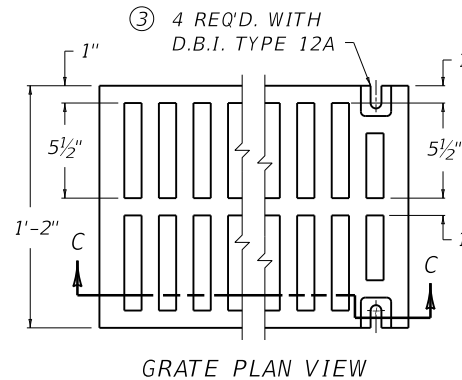
GRATE PLAN VIEW
