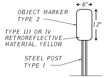
OBJECT MARKER TYPE 2 DETAIL "A" ⑦
