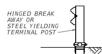
SECTION A-A POST #2
