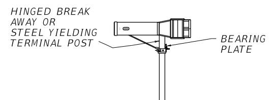
DETAIL "A" (ENLARGED VIEW P1)
