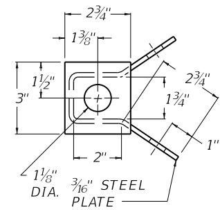
ALTERNATE NO. 2
