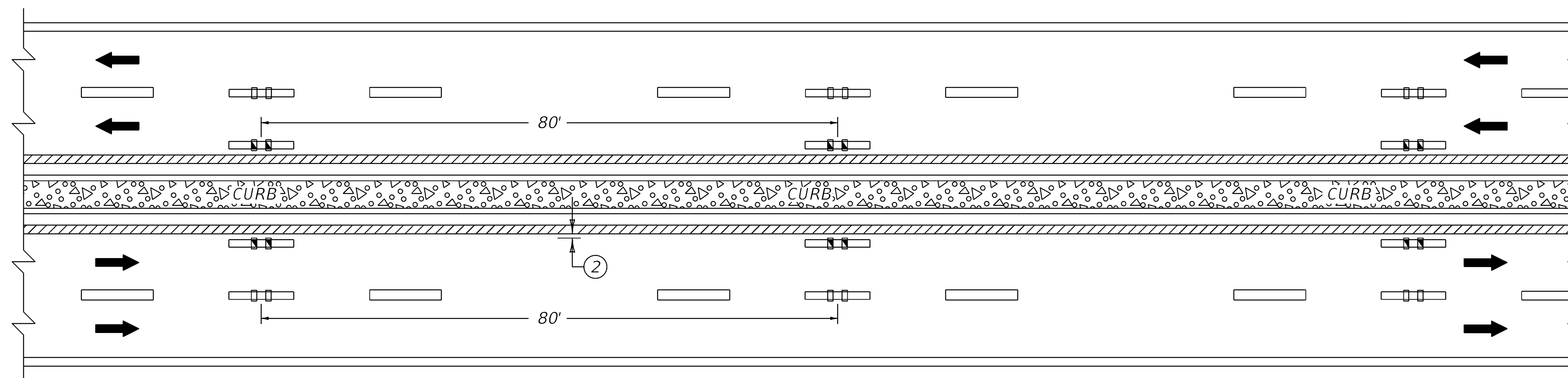
ARRANGEMENT "E" (DIVIDED HIGHWAY WITH CURB WITHIN 8' OF DRIVING LANE)
