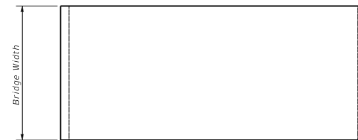
PLAN OF SUPERSTRUCTURE SLAB
