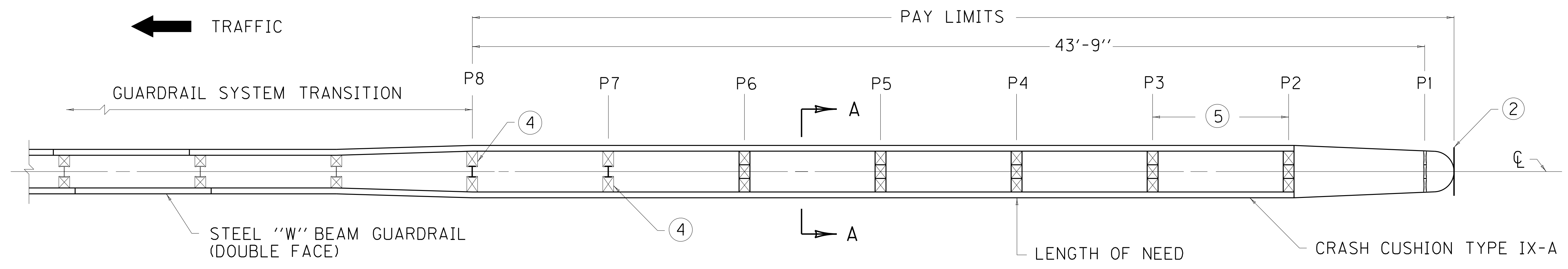
PLAN VIEW
