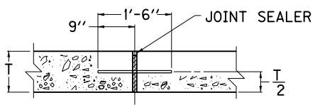
⑤ TRANSVERSE EXPANSION JOINT
