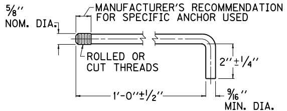
⑥ HOOK BOLT FOR USE WITH EXPANSION ANCHOR (SEE STANDARD SPECIFICATIONS FOR BASIS OF PAYMENT)
