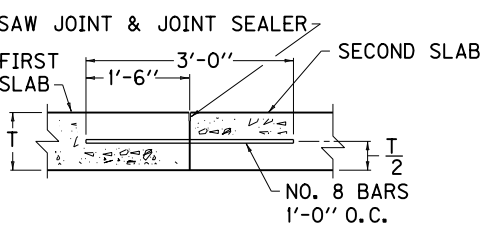
④ TRANSVERSE SAWED CONSTRUCTION JOINT
