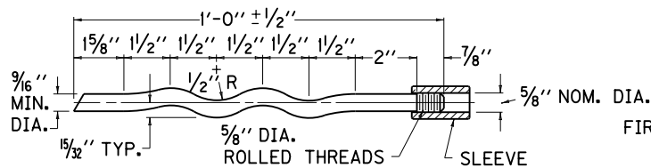
ALTERNATE 2 (FIRST SLAB) DEFORMED ANCHOR BOLT (TO BE USED WITH 8\"/>
