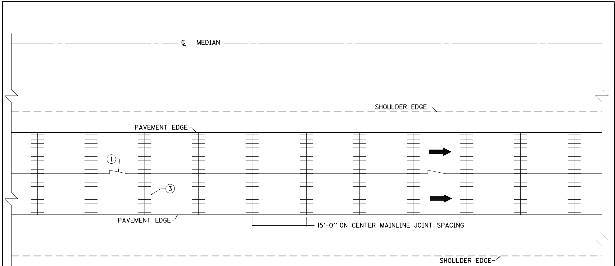
PLAN VIEW
