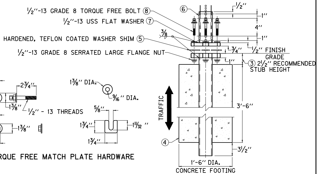
TYPE "D" SUPPORT FOR TYPE I POSTS
