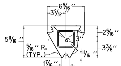
BOTTOM BASE CONCRETE STUB ②
