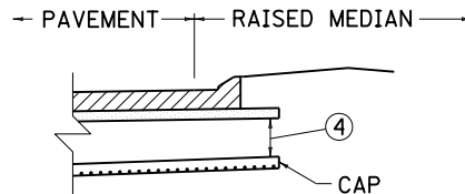
RAISED MEDIAN DETAIL "A"
