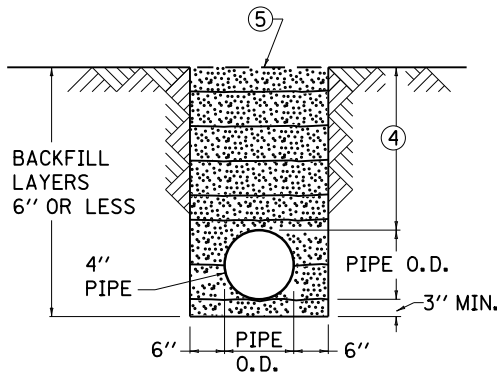
TRENCH DETAIL
