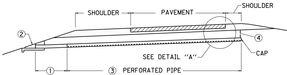
TANGENT SECTION - MULTI LANE
