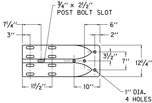
TERMINAL SECTION NO. 2
