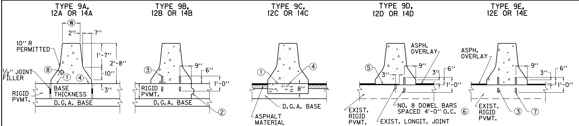
NEW RIGID PAVEMENT
