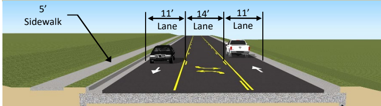
3-Lane Option – Island Ford Road – Southern Section
