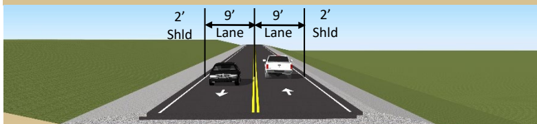
2-Lane Rural Design – Carriage Lane
