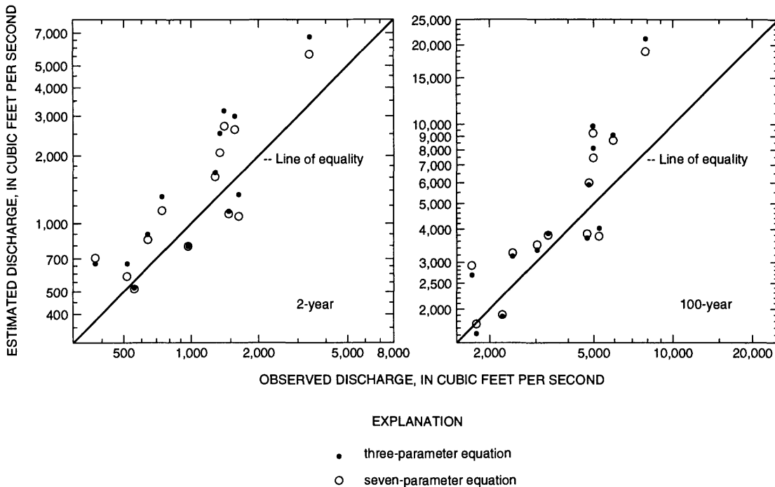
Figure 6. Comparison of 2- and 100-year observed peak discharge to peak discharges estimated using the three- and seven-parameter nationwide regression equations for urban basins in Jefferson County, Kentucky.
