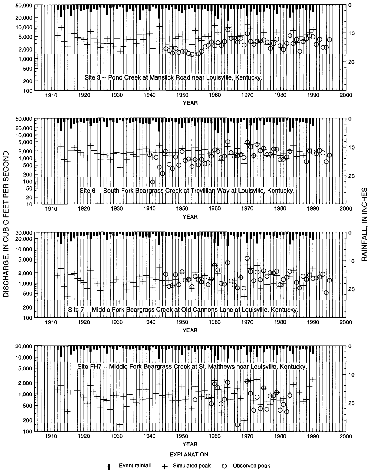
Figure 4. Simulated annual peak discharges, event rainfall, and observed annual peak discharges for selected long-term streamflow-gaging stations in Jefferson County, Kentucky.
