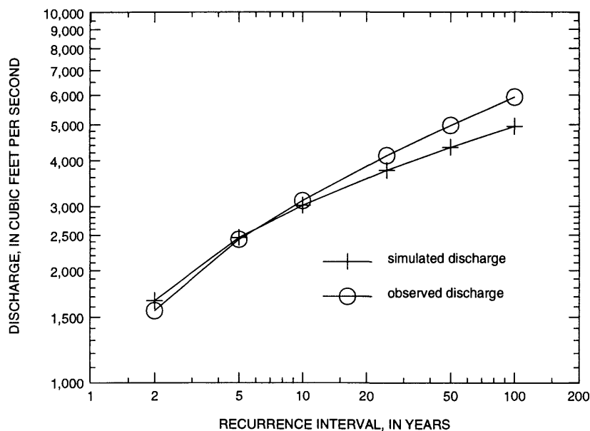
Figure 5. Comparison of peak-discharge frequencies estimated from observed and simulated annual peak discharge at South Fork Beargrass Creek at Trevilian Way at Louisville, Kentucky.
