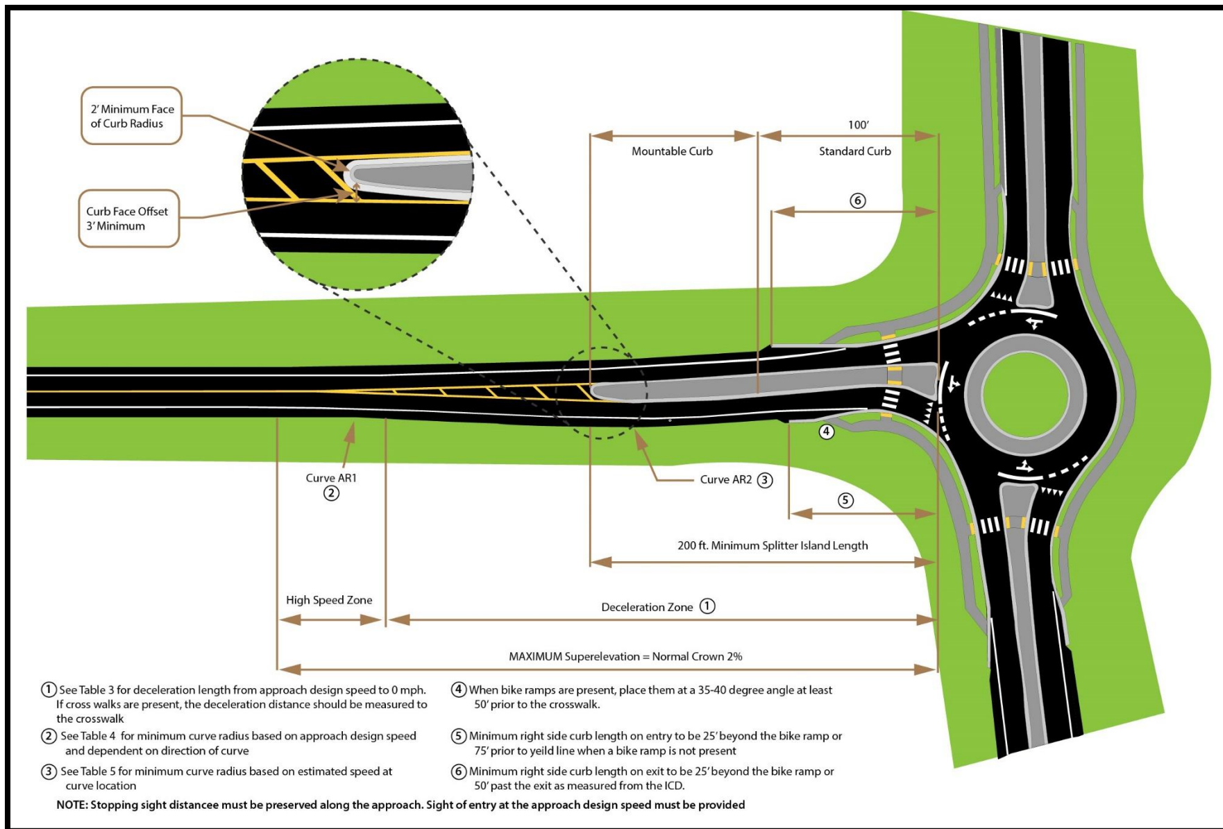
Figure 14: Curves at High-Speed Roundabout Approach
