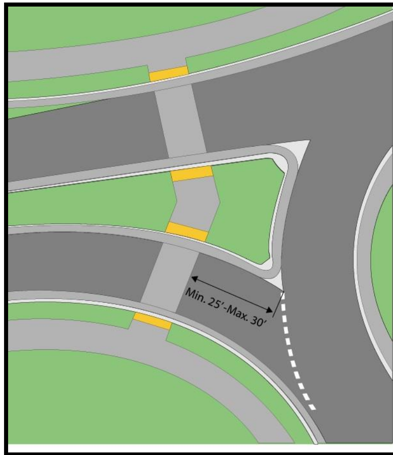
Figure 10 Angled Crosswalk in Pedestrian Refuge
