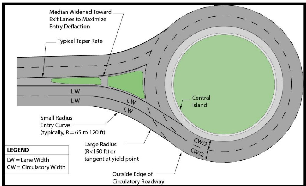
Figure 27 Entry Path Alignment
