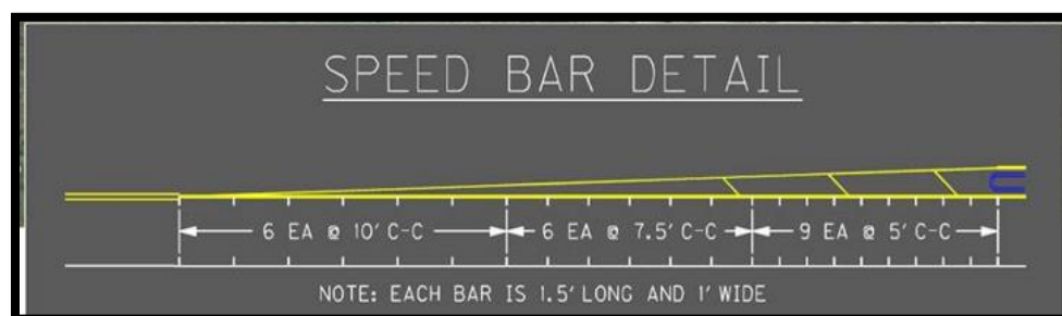
Figure 15 Optical Speed Bar Detail
