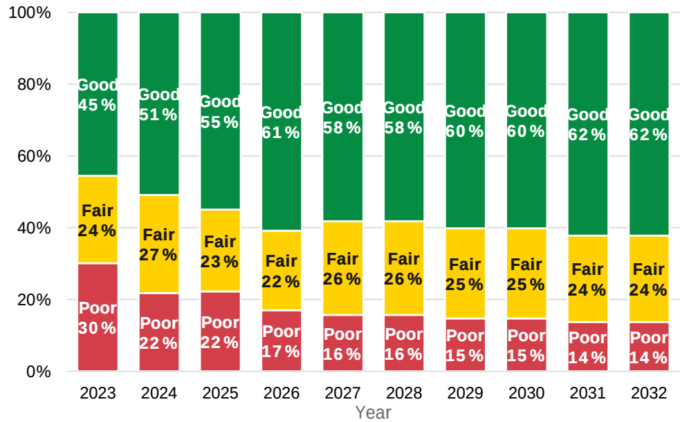
Figure 6-4: Forecasted Interstate pavement conditions based on planned investments
