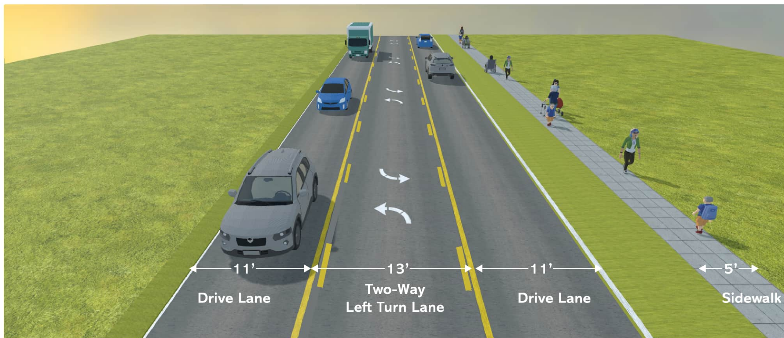
Alternate B - Typical Section
