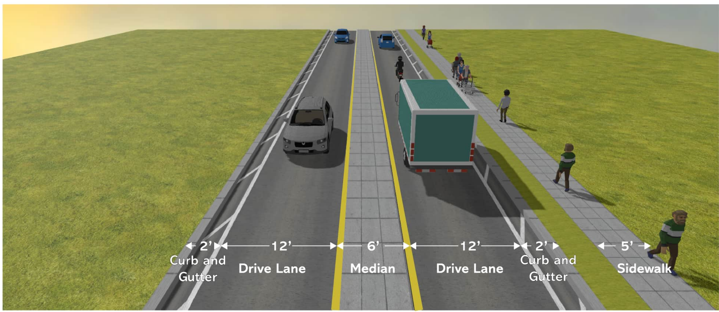
Alternate A - Typical Section
