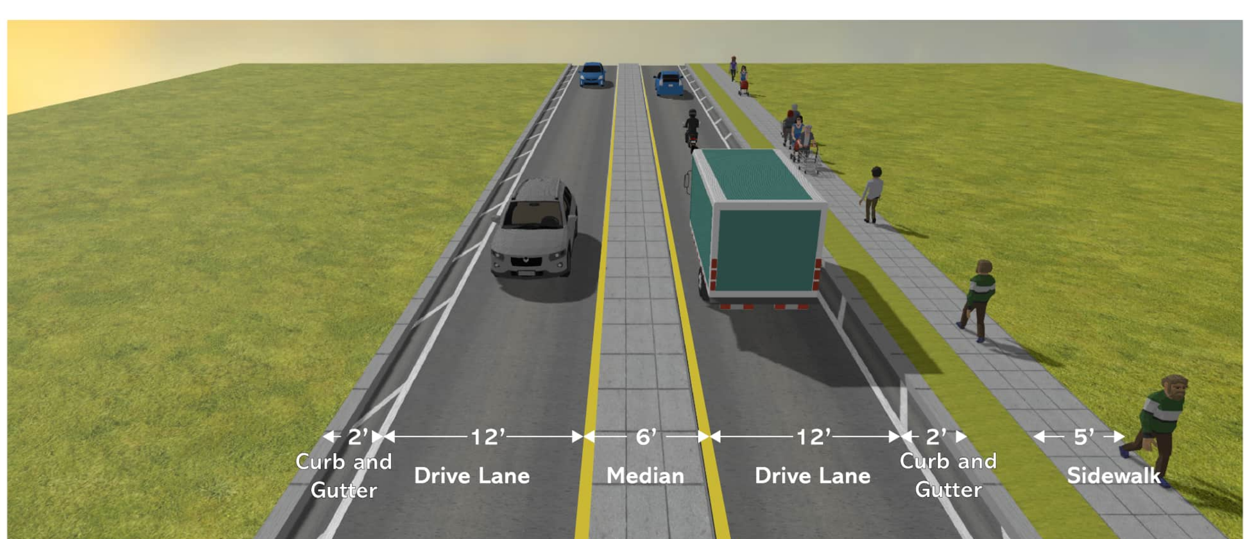
Alternate C - Typical Section
