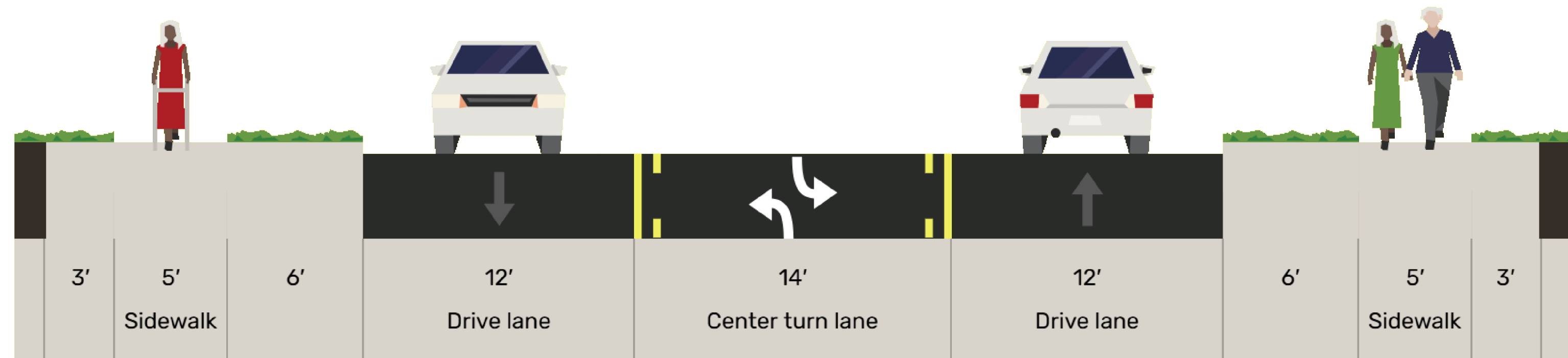
KY 1819 (Watterson Trail) - Typical Section
