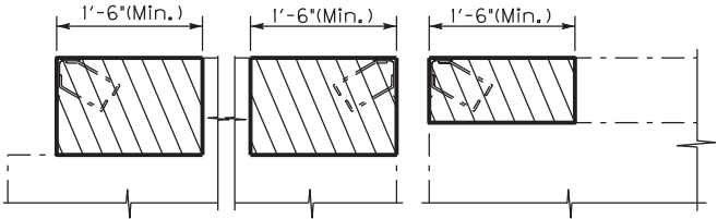
SECTION THROUGH JOINT (Existing)
