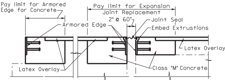
SECTION THROUGH JOINT (Proposed @ Abutment/End Bent)
